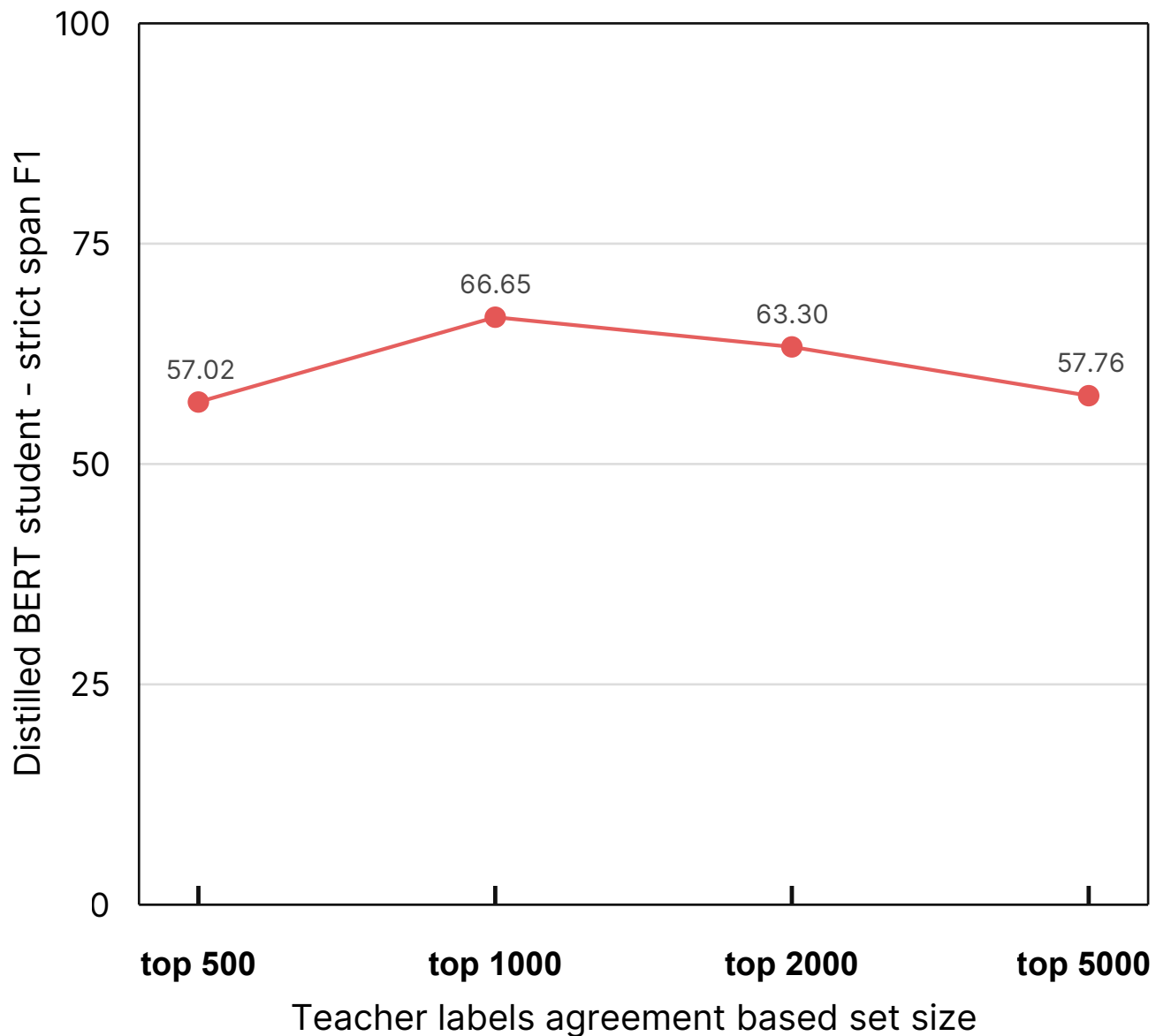
Distilled BERT performance from teacher set size
