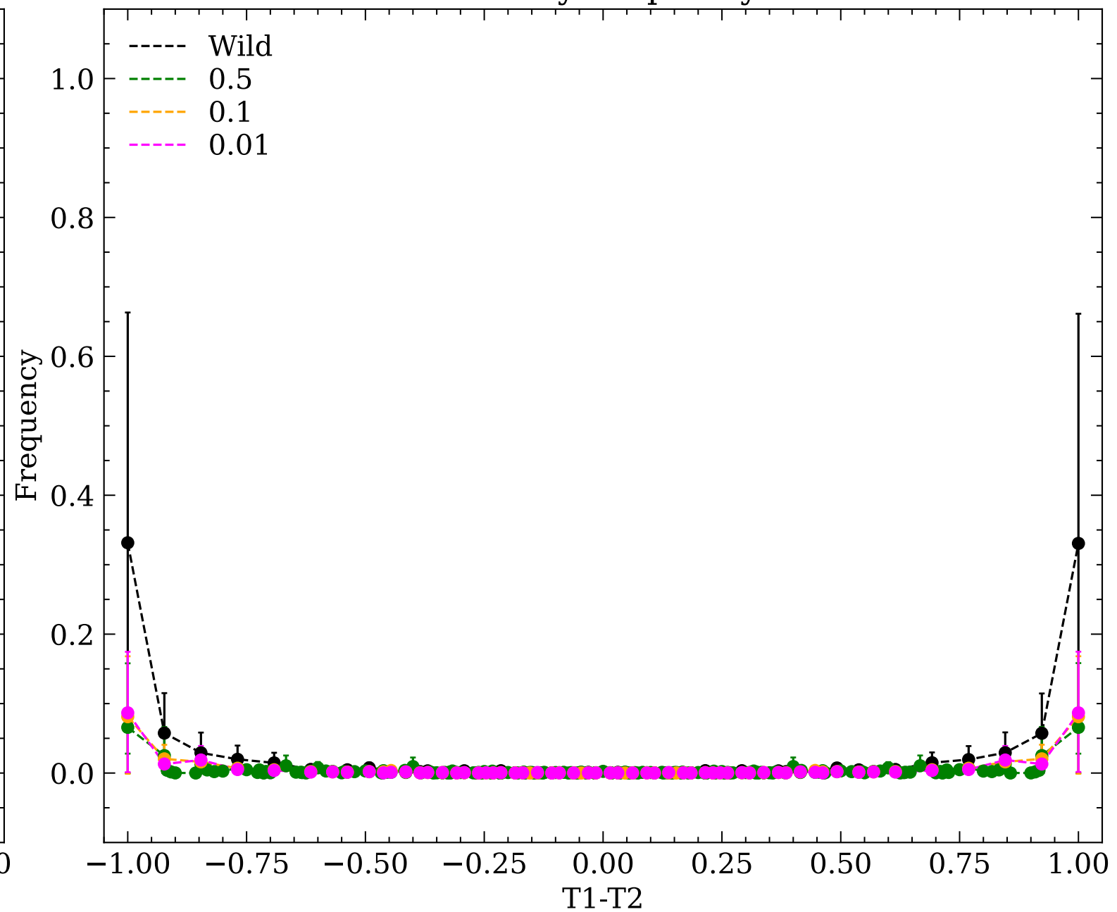
Density frequency
