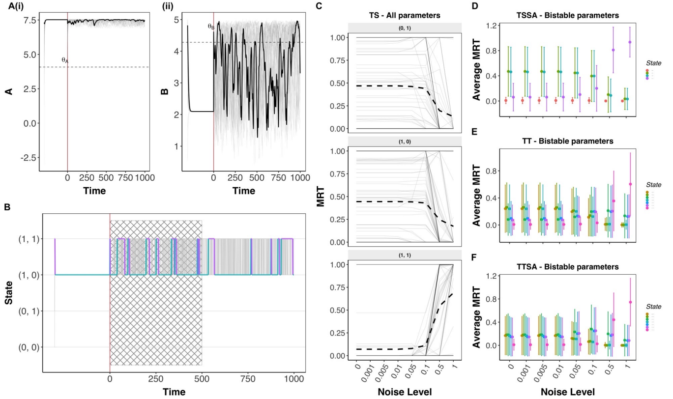
Figure 2: Effect of stationary noise on toggle switch and toggle triad networks. (A) Representative single-parameter trajectory for the TS network: (i) node A and (ii) node B expression over time (log 2 ), with the deterministic (noise-free) segment at negative time and the stochastic segment at positive time. Gray lines show all sampled initial conditions; the black line highlights one representative trajectory (the one whose switch count is closest to the population median); dashed horizontal line marks each node's discretization threshold \theta . (B) Discrete-state trace of the same parameter, colored by state for the highlighted trajectory (gray for all other initial conditions). Crosshatched region marks the discarded transient-dominated window of the stochastic segment. (C) MRT of each state across noise levels. Each panel corresponds to the state indicated by its label. Grey lines show a random sample of 100 parameter-set trajectories (out of the full population, shown for legibility); the black dashed line shows the mean across the full parameter population, not just the sampled 100. Darker or apparently solid grey segments result from the overlap of multiple trajectories and do not denote a separate category. (D–F) MRT vs. noise level for TSSA (D), TT (E), and TTSA (F) bistable parameter sets, colored by state (top 4 states shown for TSSA, top 7 for TT/TTSA), mean \pm SD across parameter sets.
