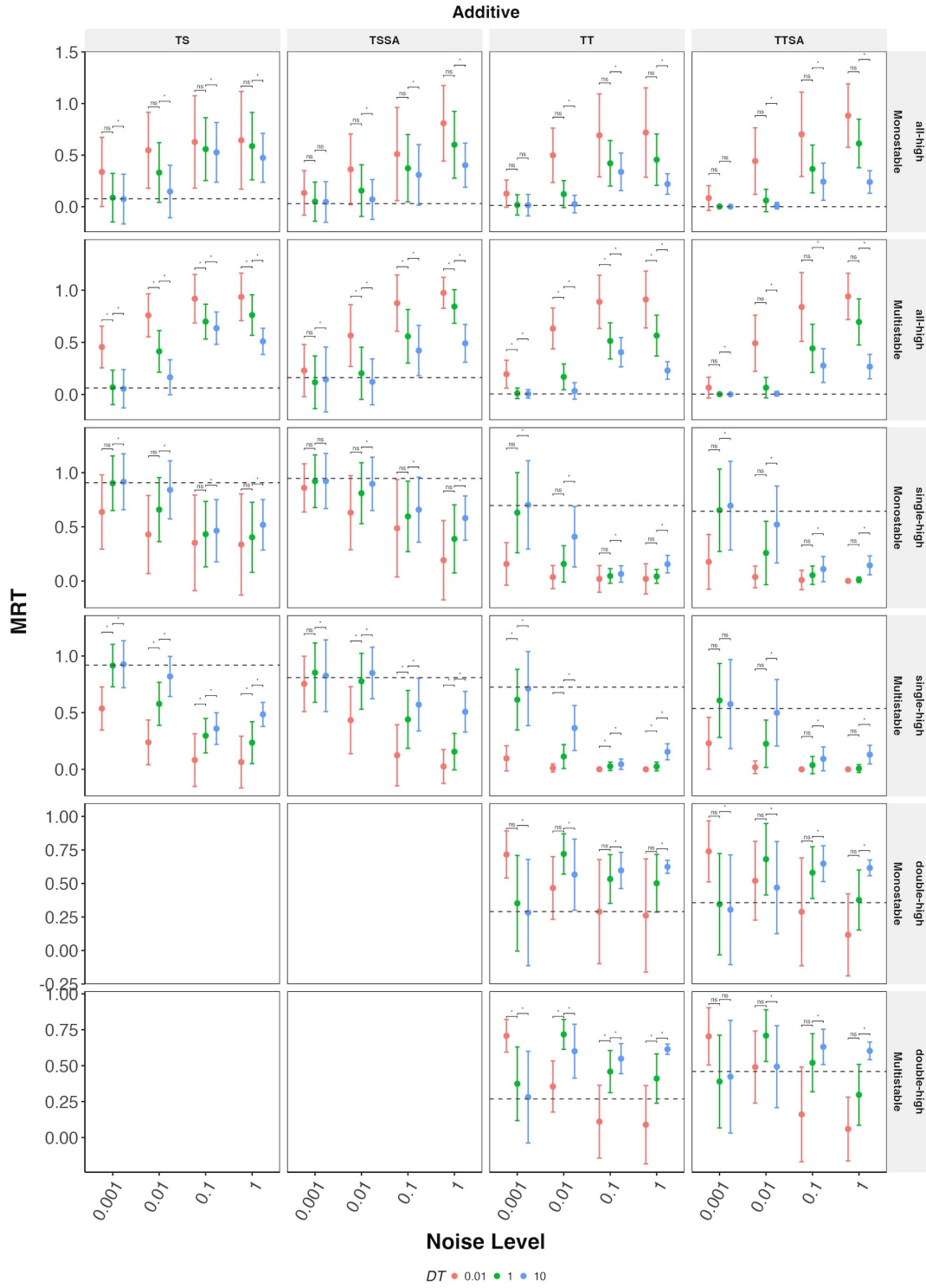
Figure S1: Comparison of MRTs for additive noise simulated at different values of dt
