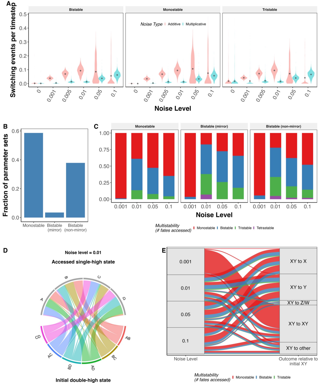
Figure 6: Fate resolution of progenitor state under multiplicative noise (A) Distribution of switching-event counts by noise level (Additive vs. Multiplicative), after excluding the initial burn-in window. (B) Frequency of the three deterministic stability classes among double-high parameter sets. (C) For each stability class, the fraction of parameter sets accessing 1 (Monostable), 2 (Bistable), or 3+ (Tristable/Tetrastable) distinct single-high fates under noise. (D) Circular chord diagram of double-high \rightarrow single-high MRT flow among monostable double-high parameter sets, at \sigma = 0.01 . (E) Noise-level \rightarrow outcome alluvial for the pooled monostable double-high population (outcomes labeled relative to the initial double-high state XY, e.g. “XY to X”), colored by the multistability classification from panel C.
