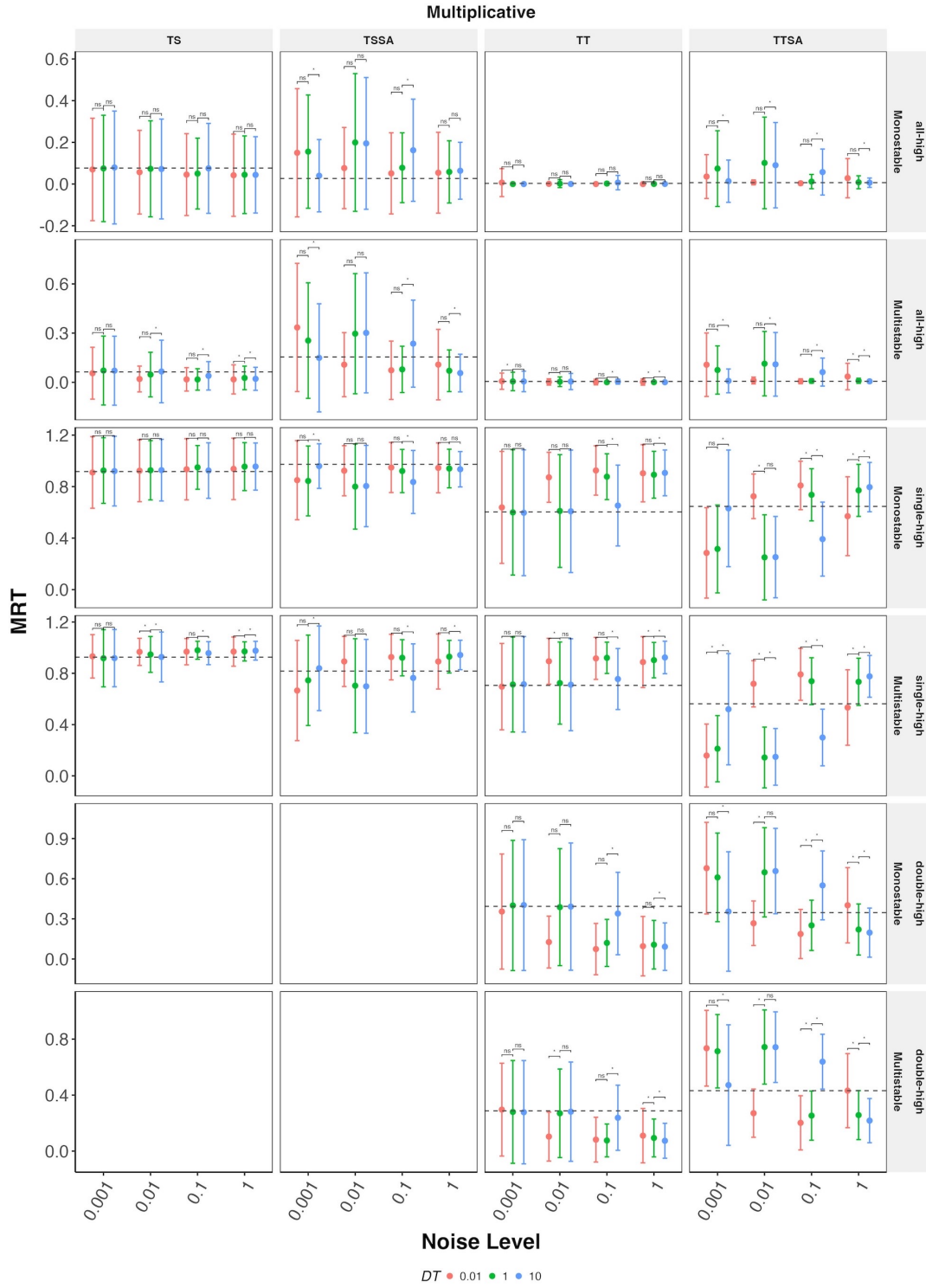
Figure S2: Comparison of MRTs for multiplicative noise simulated at different values of dt
