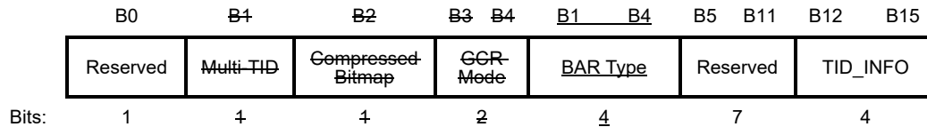
Figure 9-36—BAR Control field format
