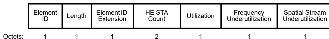
Figure 9-788ad—HE BSS Load element format
