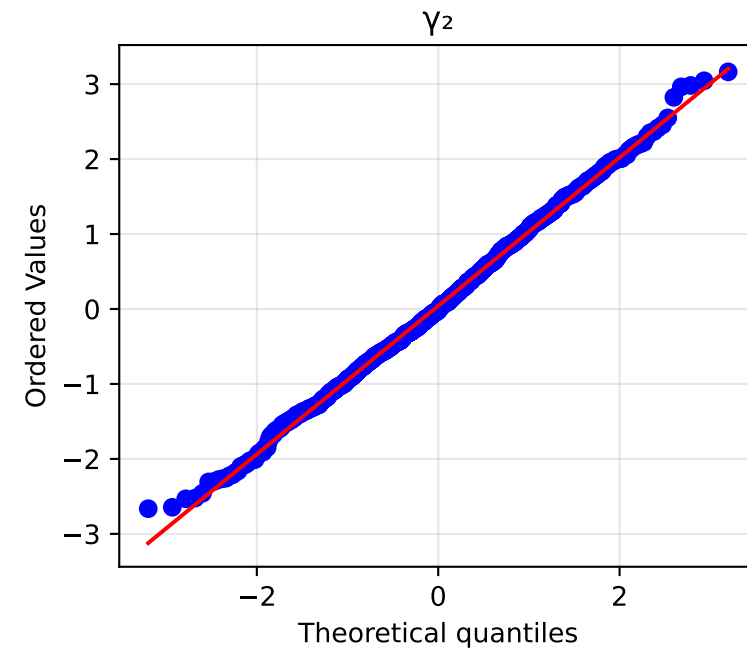
Q-Q plots of ML z-scores against N(0,1)
