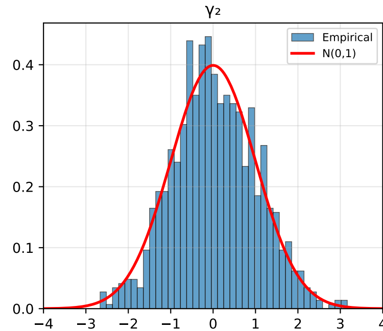
ML z-scores with N(0,1) overlay
