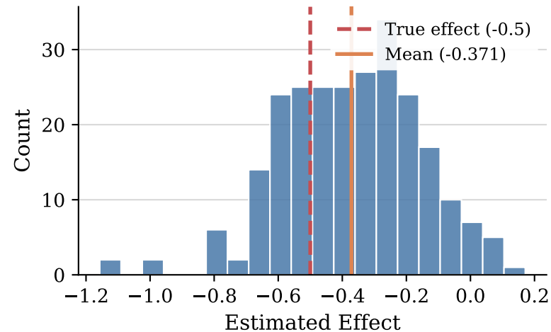
Cross-sectional OLS
