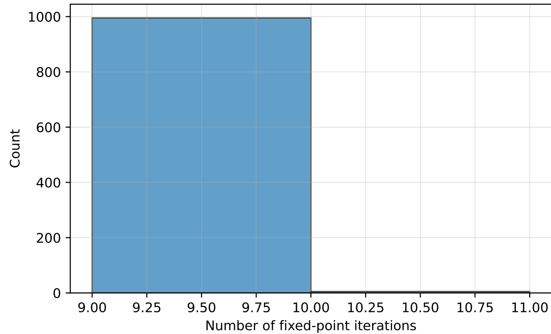
Fixed-Point Iteration Counts
