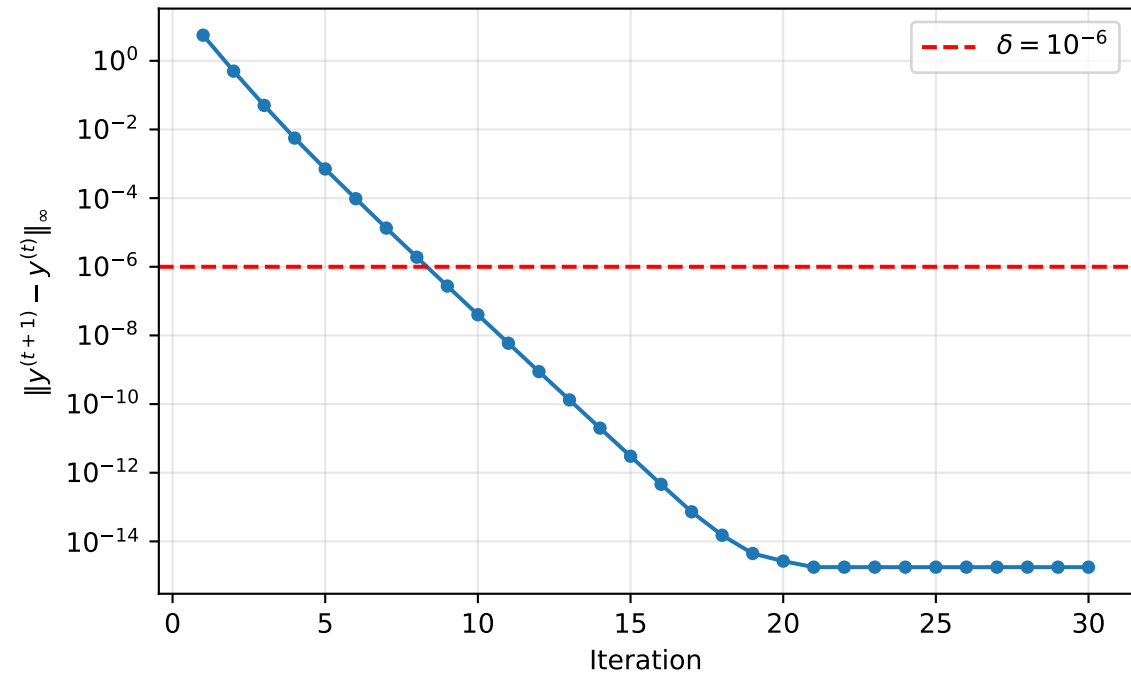
Convergence Trace (single replication)
