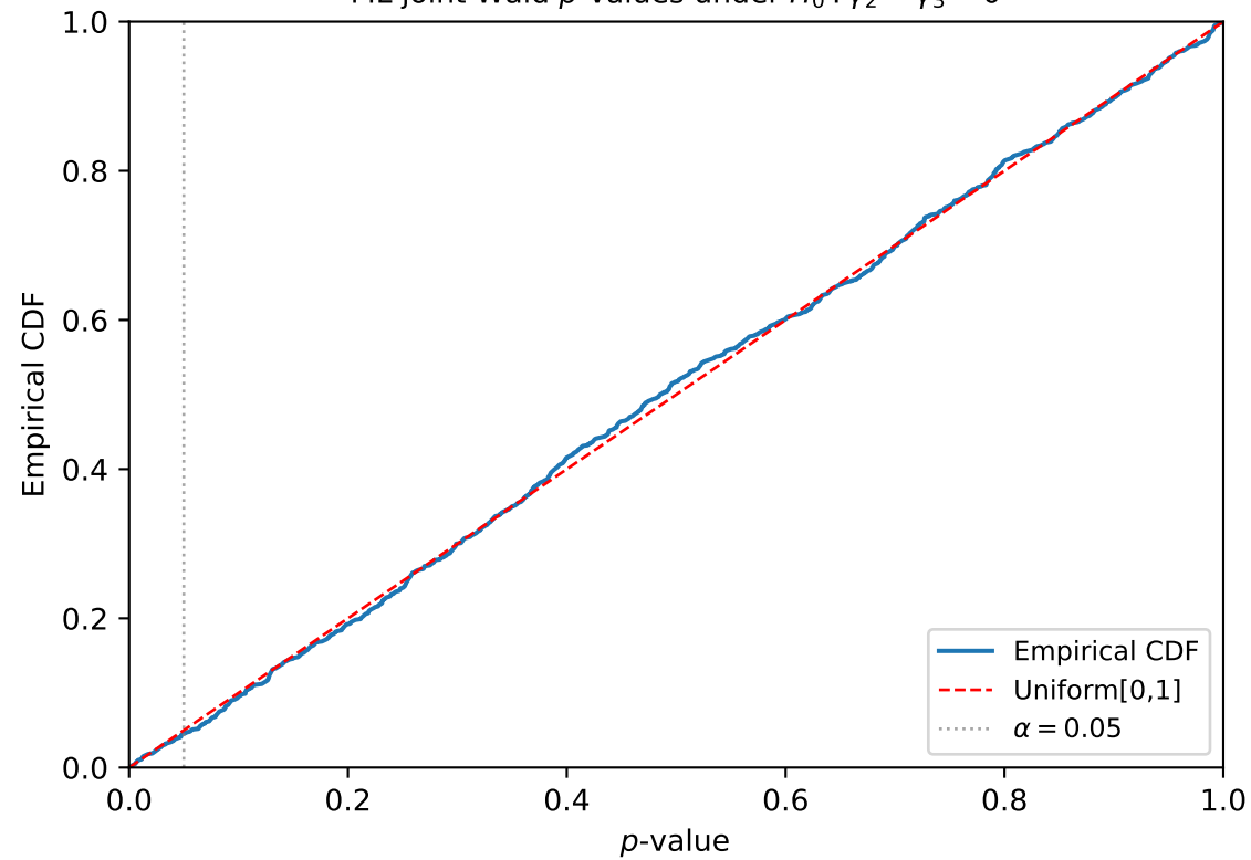
ML joint Wald p -values under H_0 : \gamma_2 = \gamma_3 = 0
