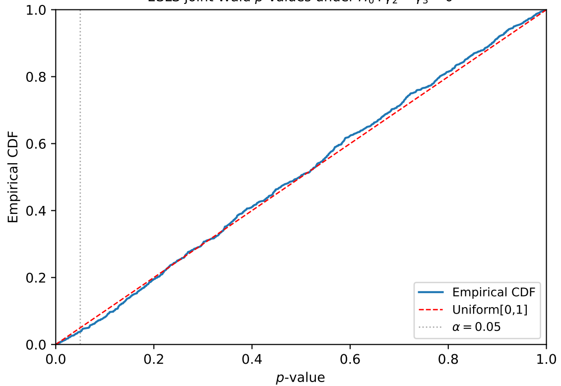
2SLS joint Wald p -values under H_0 : \gamma_2 = \gamma_3 = 0
