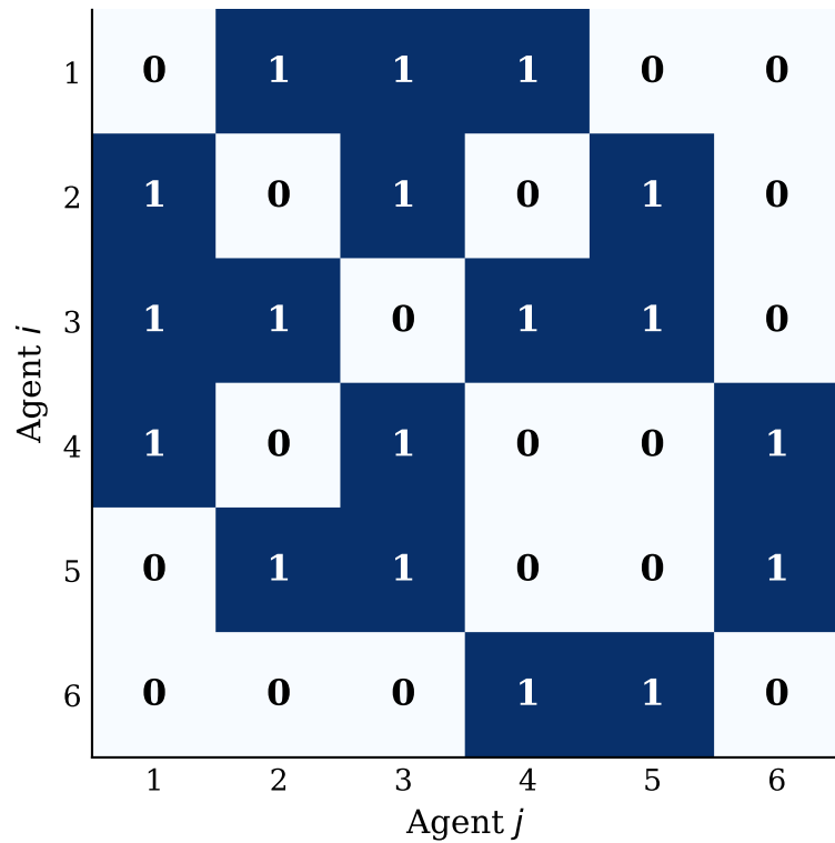
Adjacency Matrix A
