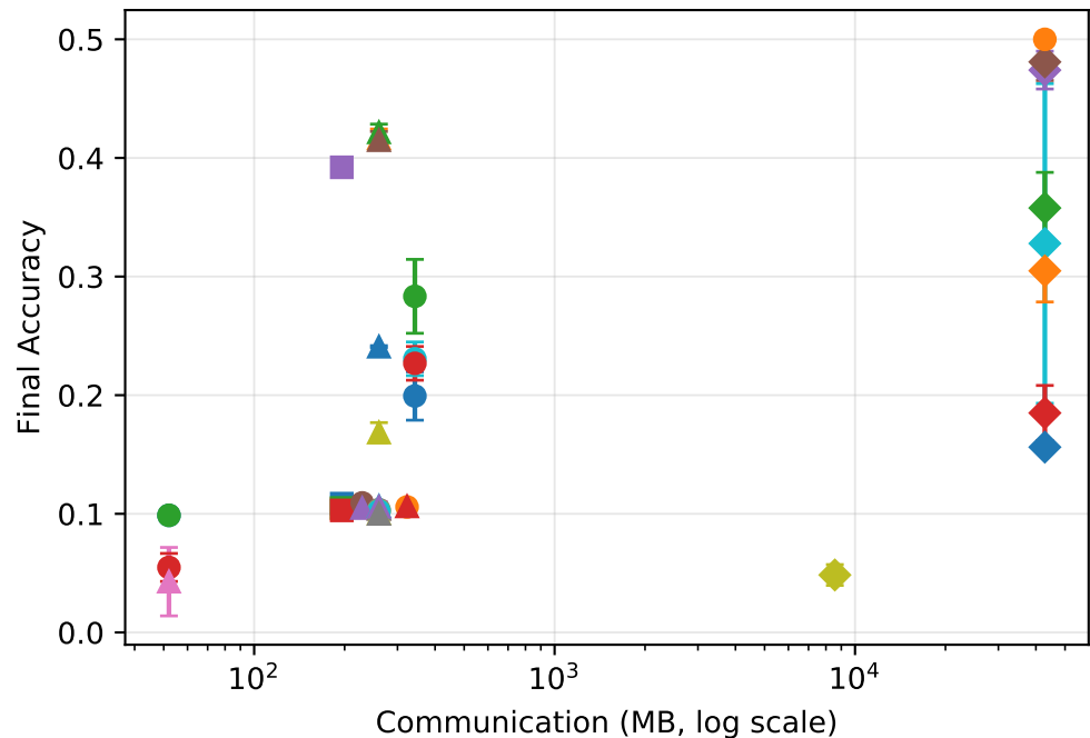
(b) Accuracy vs Communication
