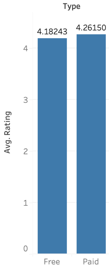
Rating_Free_vs_Paid
