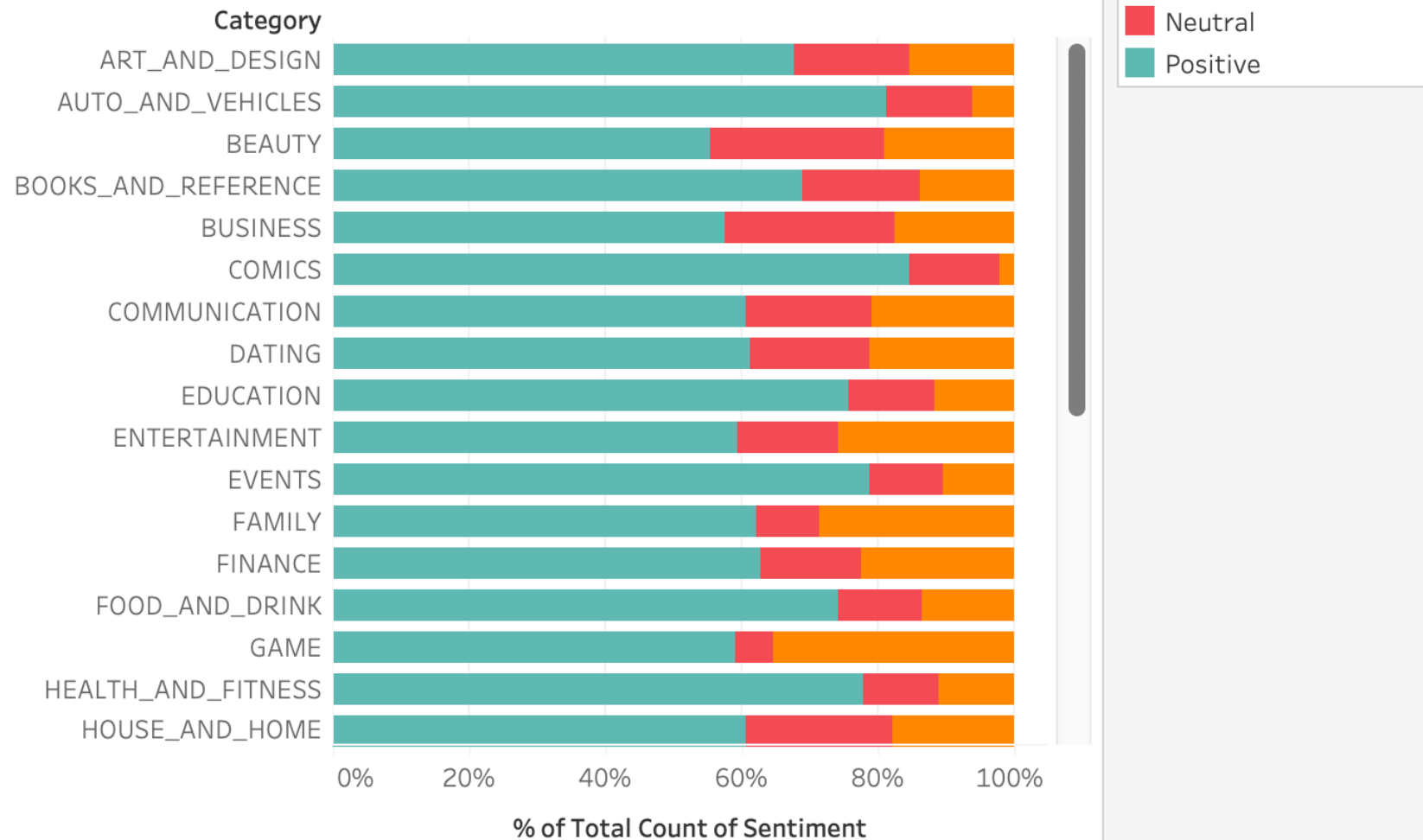
Sentiment_by_Category
