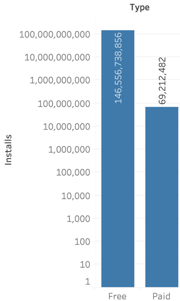
Installs_Free_vs_Paid
