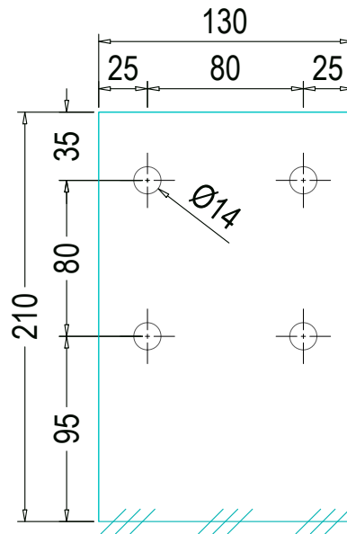
DETAILS OF PC210*6 ( THICKNESS 6mm ) Qty: 24Nos
