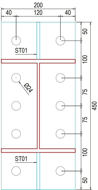
DETAILS OF CP450x200x20 (20mm Thickness) Qty: 36Nos
