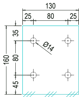
DETAILS OF PC160*6 ( THICKNESS 6mm ) Qty: 120Nos
