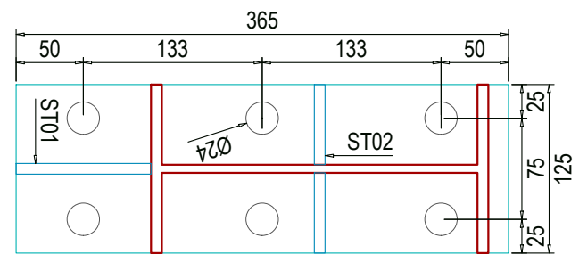
DETAILS OF CP365x125x16 (16mm Thickness) Qty: 08Nos
