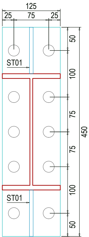
DETAILS OF CP450x125x16 (16mm Thickness) Qty: 08Nos
