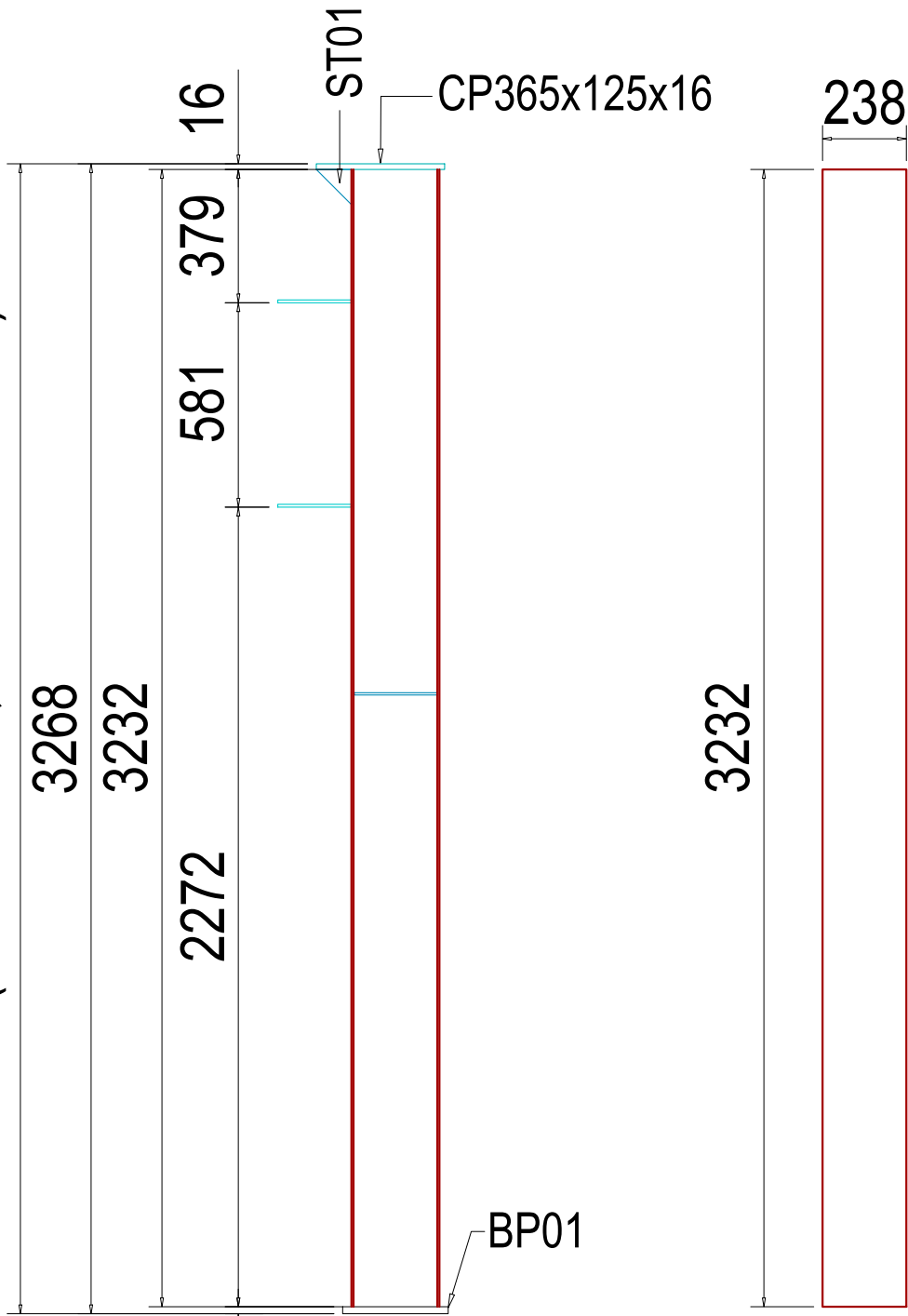
DETAIL OF SC101 (04 PCS) CUTTING WEB OF SC01
