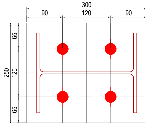
DETAILS OF BP01 (THICK: 20mm );Total: 16Nos.
