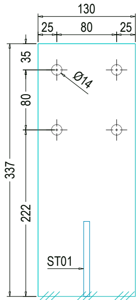
DETAILS OF PC337*8 ( THICKNESS 8mm ) Qty: 04Nos
