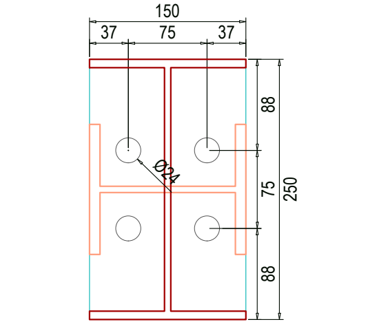
DETAILS OF CP250x150x16 (16 mm Thickness) Qty: 08Nos
