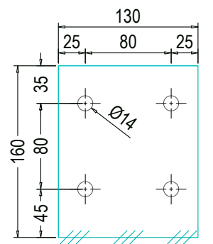
DETAILS OF PC160*6 (THICKNESS 6mm) Qty: 120Nos
