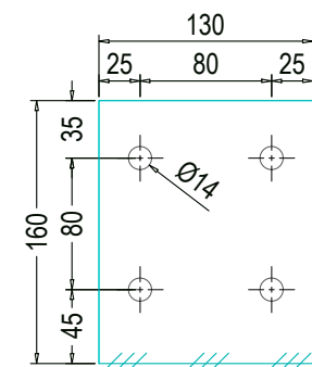
DETAILS OF PC160*6 ( THICKNESS 6mm ) Qty: 120Nos
