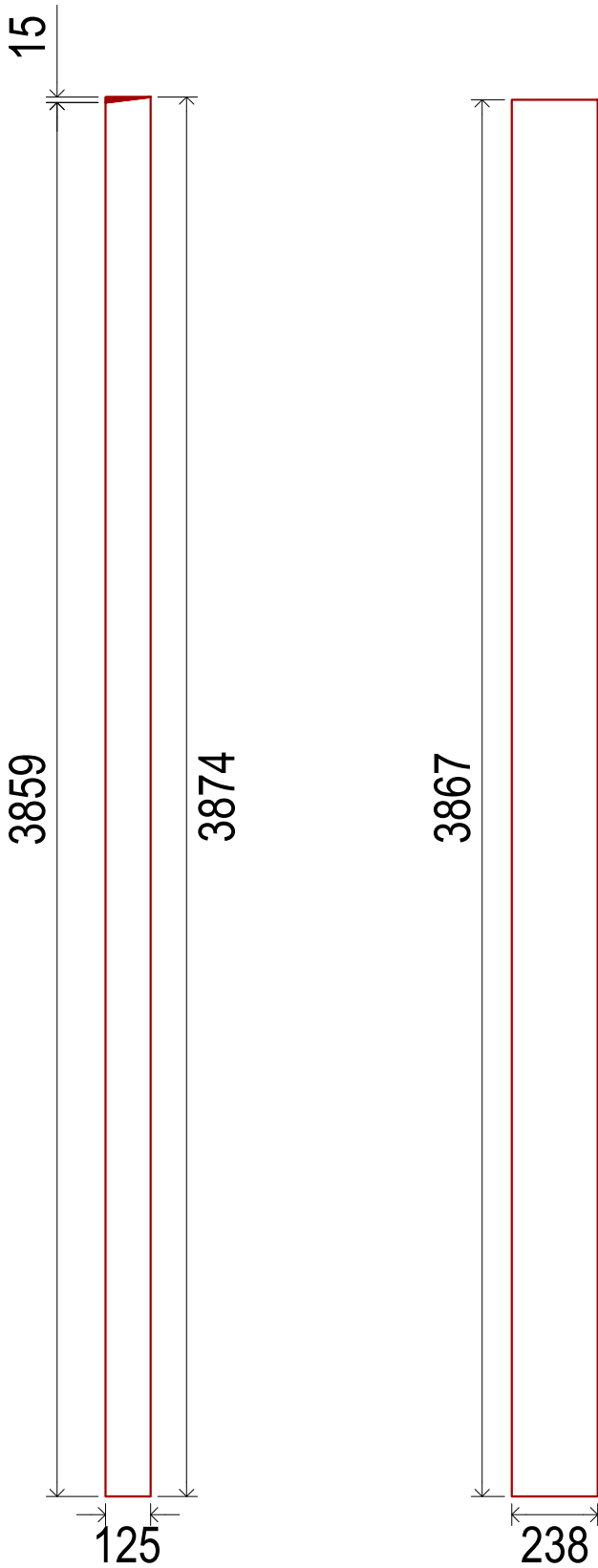
CUTTING WEB OF SC102
