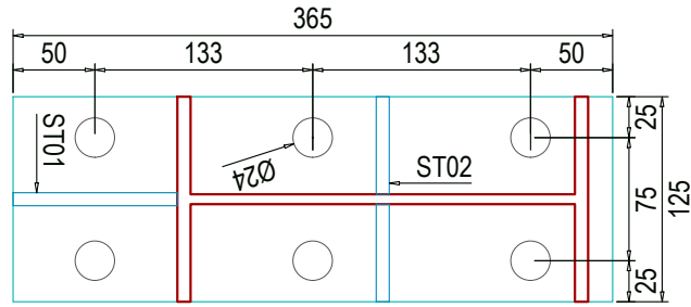
DETAILS OF CP365x125x16 (16mm Thickness) Qty: 08Nos
