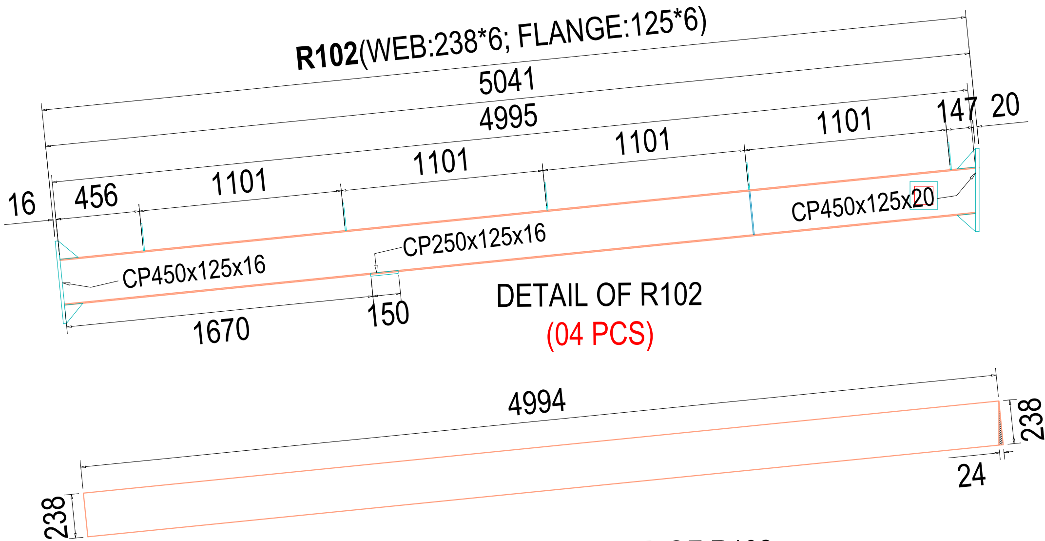
CUTTING WEB OF R102
