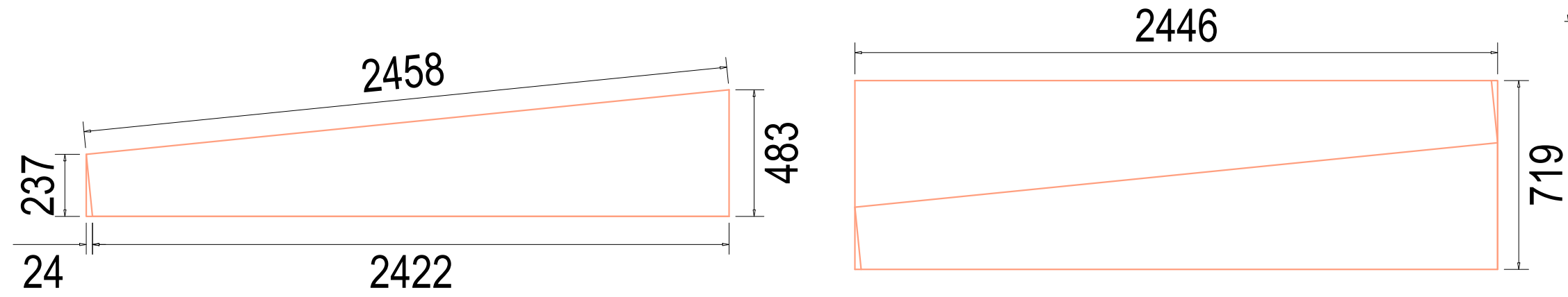
DETAILS OF PC160*6 ( THICKNESS 6mm ) Qty: 120Nos
