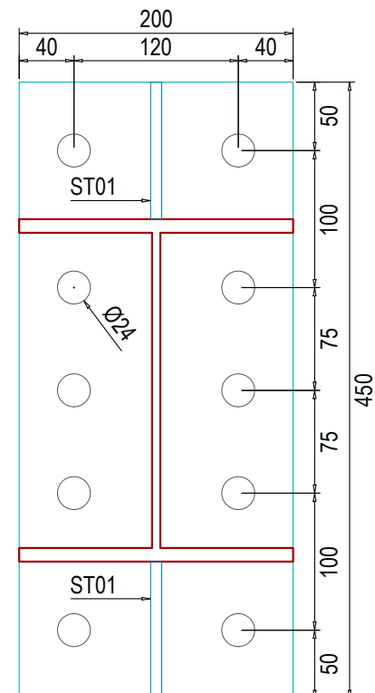
DETAILS OF CP450x200x20 (20mm Thickness) Qty: 36Nos
