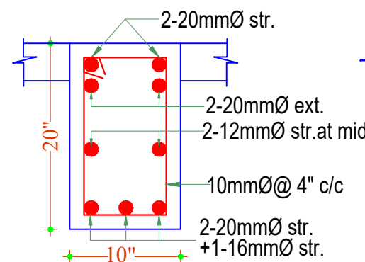
SECTION: FB101-FB101
