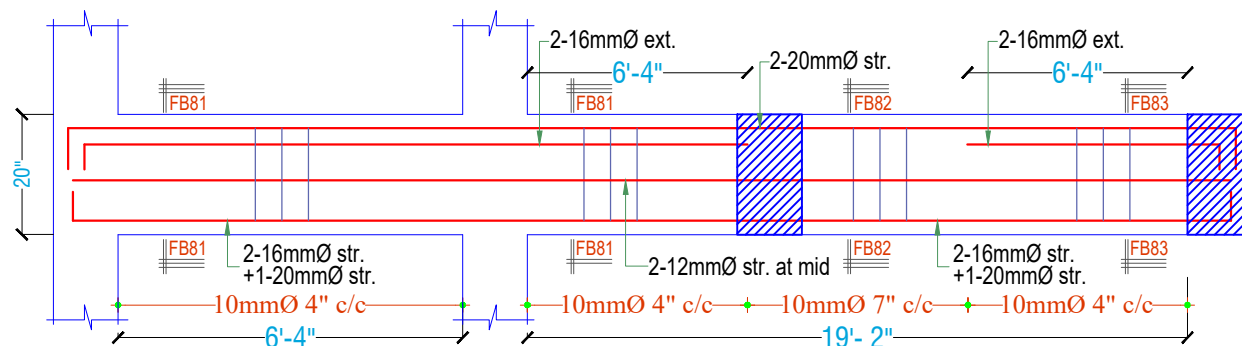
LONG SECTION OF FLOOR BEAM-8 (10"X20")
