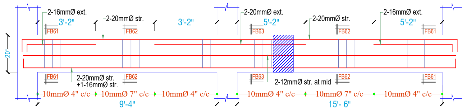
LONG SECTION OF FLOOR BEAM-6 (10"X20")
