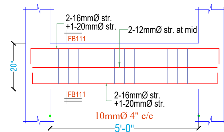
LONG SECTION OF FLOOR BEAM-11 (10"X20")
