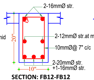
SECTION: FB12-FB12
