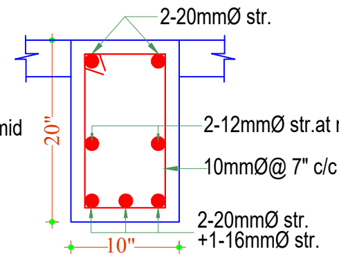
SECTION: FB102-FB102
