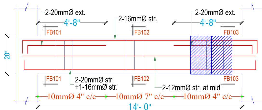
LONG SECTION OF FLOOR BEAM-10 (10"X20")
