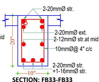
SECTION: FB33-FB33
