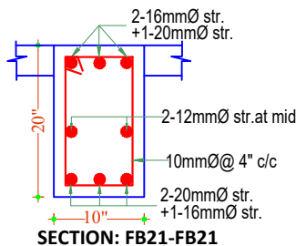
SECTION: FB21-FB21
