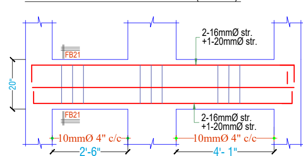
LONG SECTION OF FLOOR BEAM-2 (10"X20")
