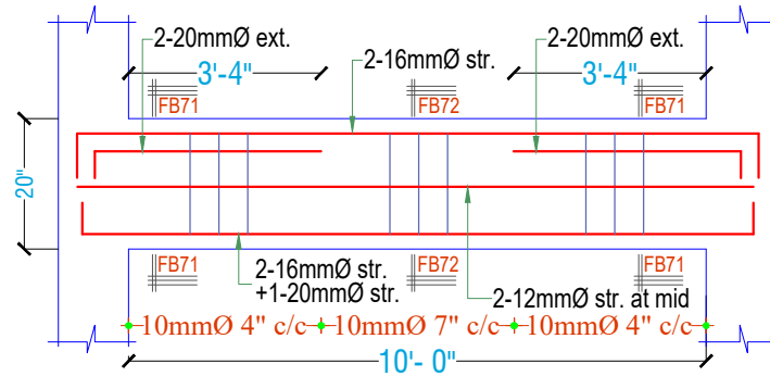
LONG SECTION OF FLOOR BEAM-7 (10"X20")
