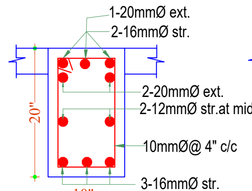
SECTION: FB91-FB91
