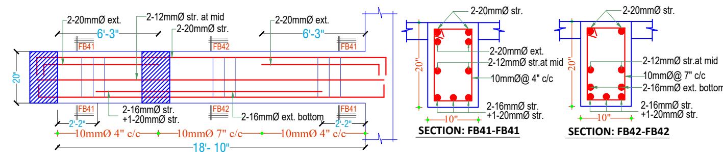
LONG SECTION OF FLOOR BEAM-4 (10"X20")
