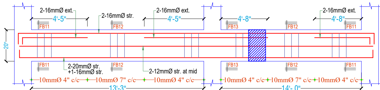
LONG SECTION OF FLOOR BEAM-1 (10"X20")
