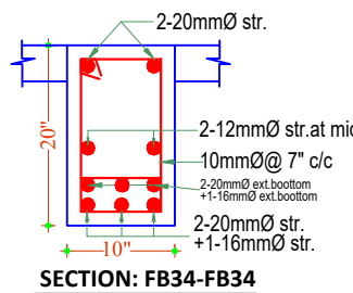
SECTION: FB34-FB34
