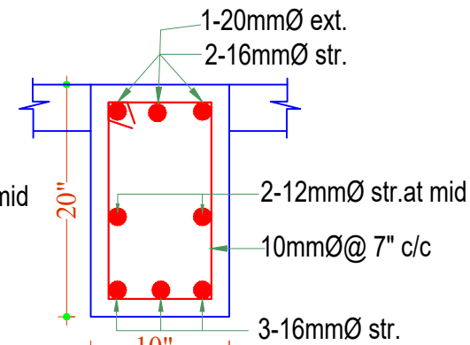
SECTION: FB92-FB92
