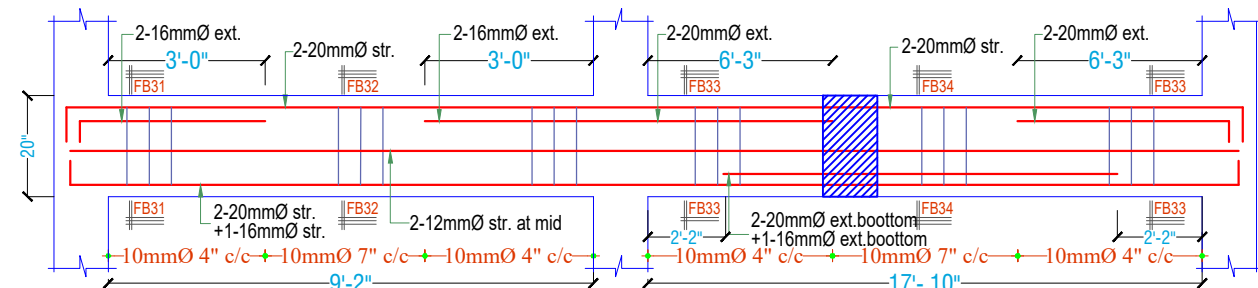
LONG SECTION OF FLOOR BEAM-3 (10"X20")
