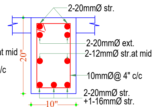
SECTION: FB103-FB103
