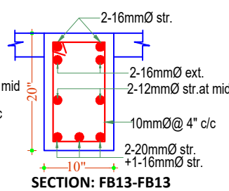
SECTION: FB13-FB13
