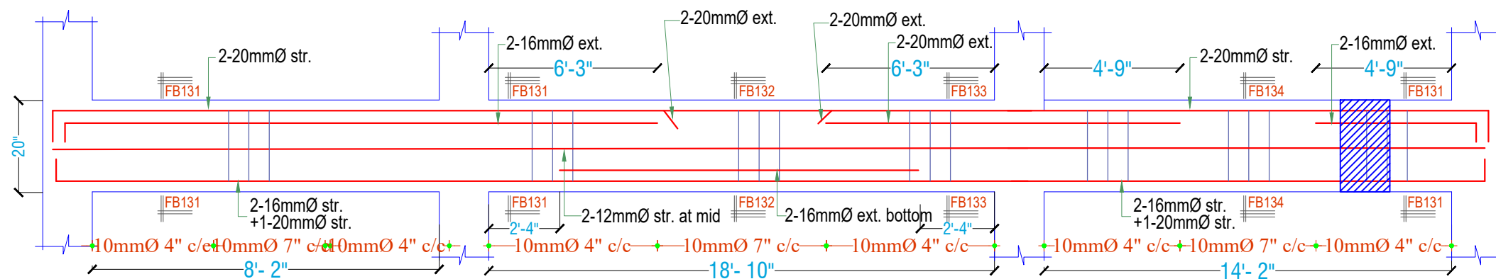
LONG SECTION OF FLOOR BEAM-13 (10"X20")
