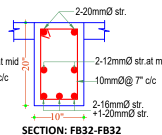
SECTION: FB32-FB32
