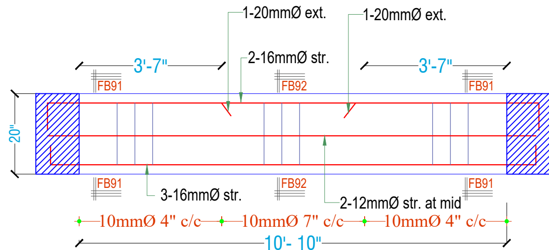
LONG SECTION OF FLOOR BEAM-09 (10"X20")
