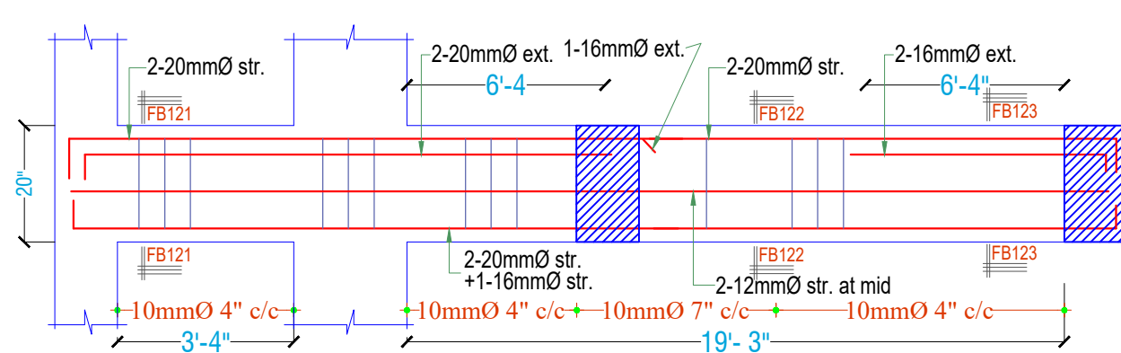
LONG SECTION OF FLOOR BEAM-12 (10"X20")
