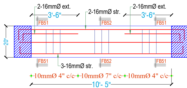
LONG SECTION OF FLOOR BEAM-5 (10"X20")
