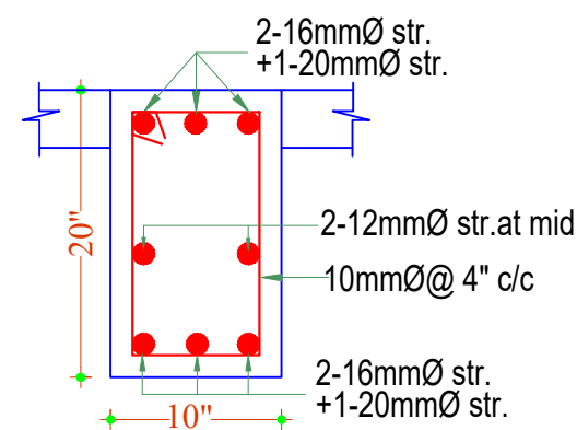
SECTION: FB111-FB111
