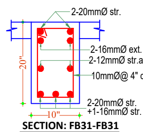
SECTION: FB31-FB31
