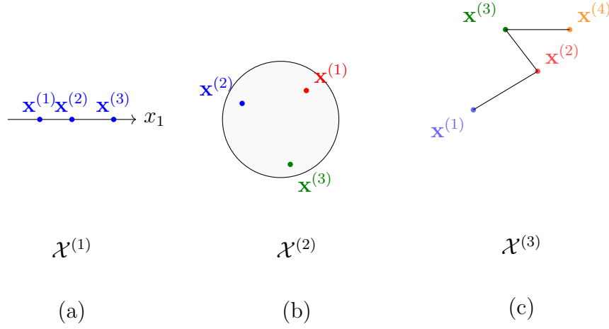
Fig. 87. Three different feature spaces. (a) A linear space \mathcal{X}^{(1)} = \mathbb{R} . (b) A bounded convex set \mathcal{X}^{(2)} \subseteq \mathbb{R}^2 . (c) A discrete space \mathcal{X}^{(3)} whose elements are nodes of an undirected graph.
