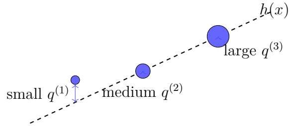
Fig. 127. Sample weighting assigns each data point of a training set a weight q^{(r)} . Assigning a small weight (such as q^{(1)} in this example) to a data point decreases its influence on the hypothesis learned via solving (19).
