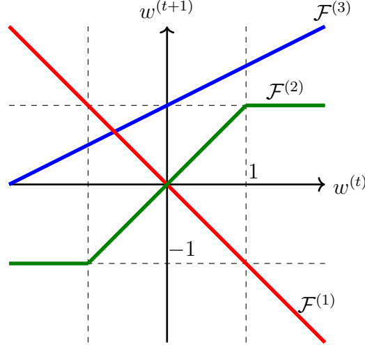
Fig. 26. Example of a non-expansive operator \mathcal{F}^{(1)} , a firmly non-expansive operator \mathcal{F}^{(2)} , and a contractive operator \mathcal{F}^{(3)} .
