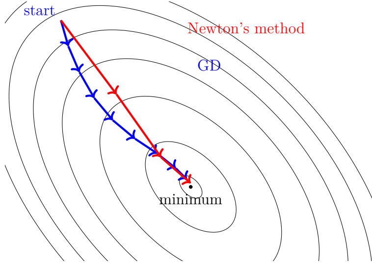
Fig. 47. Comparison of GD (blue) and Newton's method (red) paths toward the minimum of a loss function.
