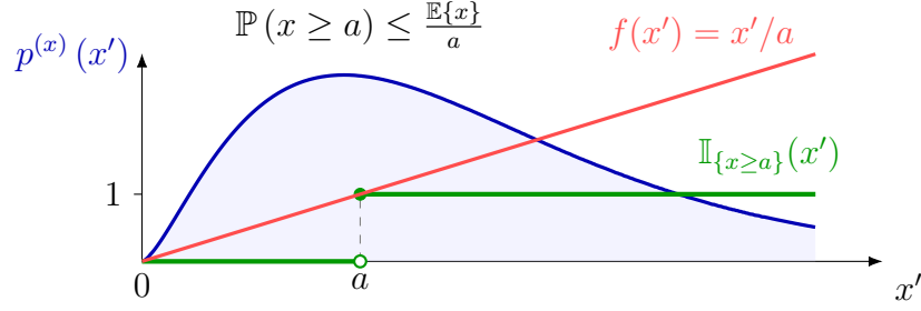
Fig. 40. The expectation \mathbb{E}\{x\} and the probability \mathbb{P}(x \geq a) of a nonnegative RV x with a pdf p^{(x)}(\cdot) can be obtained via Lebesgue integrals of f(x') = x'/a and g(x') = \mathbb{I}_{\{x \geq a\}}(x') , respectively.
