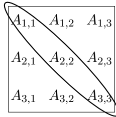
Fig. 60. The trace \text{tr}(\mathbf{A}) of a 3 \times 3 matrix \mathbf{A} \in \mathbb{R}^{3 \times 3} is the sum of three main diagonal entries A_{1,1} , A_{2,2} , A_{3,3} .
