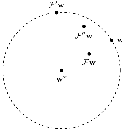
Fig. 48. The result of applying a contractive operator \mathcal{F} , a non-expansive operator \mathcal{F}' , and a firmly non-expansive operator \mathcal{F}'' . These operators have the common fixed point \mathbf{w}^* .
