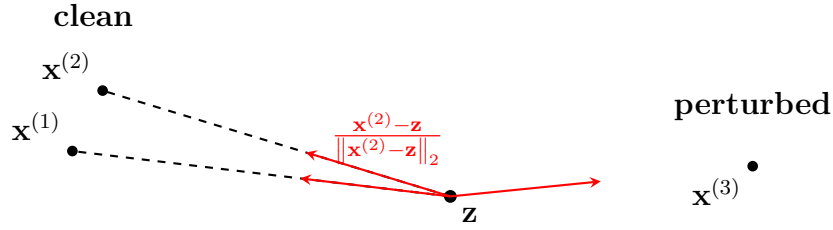
Fig. 30. Consider a solution \mathbf{z} of (5) that does not coincide with any of the input vectors. The optimality condition for (5) requires that the unit vectors from \mathbf{z} to the input vectors sum to zero.
