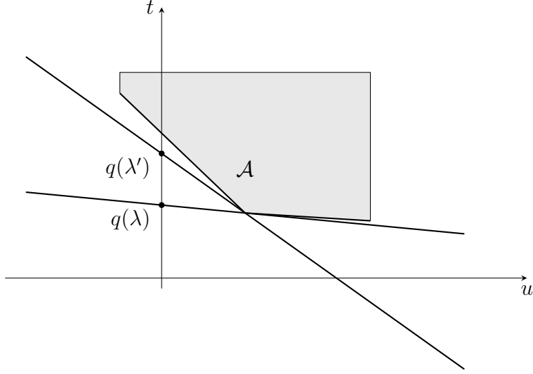
Fig. 22. The dual problem of a constrained optimization problem is to find a supporting hyperplane with the largest vertical intercept [23, Sec. 5.3].
