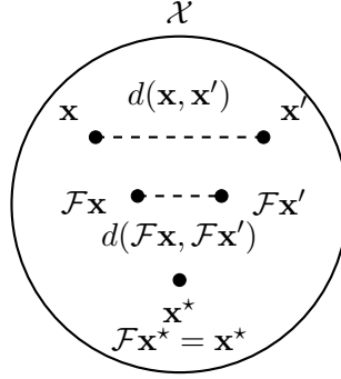
Fig. 10. A contractive operator \mathcal{F} : \mathcal{X} \rightarrow \mathcal{X} has a unique fixed point \mathbf{x}^* with \mathcal{F}\mathbf{x}^* = \mathbf{x}^* . For any two points \mathbf{x}, \mathbf{x}' in the same space, the distance between their images \mathcal{F}\mathbf{x} and \mathcal{F}\mathbf{x}' is strictly smaller.
