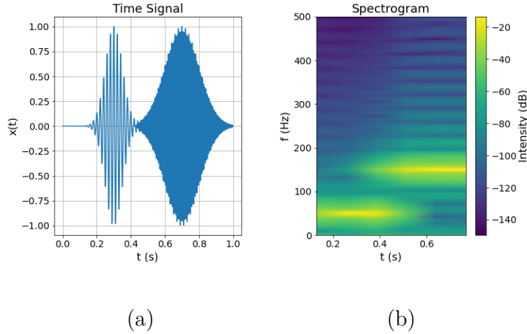
Fig. 130. (a) A time signal consisting of two modulated Gaussian pulses. (b) An intensity plot of the spectrogram.
