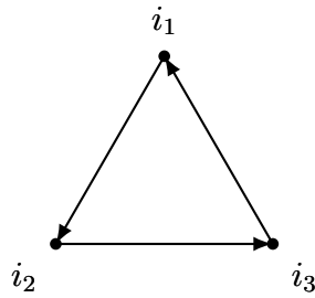
Fig. 20. A directed cycle consisting of three nodes connected in a closed loop.
