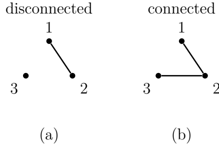
Fig. 8. (a) A graph that is disconnected. (b) A graph that is connected.
