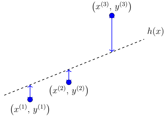
Fig. 82. ERM learns a hypothesis h \in \mathcal{H} out of a model \mathcal{H} by minimizing the average loss (or empirical risk) 1/m \sum_{r=1}^m L((\mathbf{x}^{(r)}, y^{(r)}), h) incurred on a training set \mathcal{D} .
