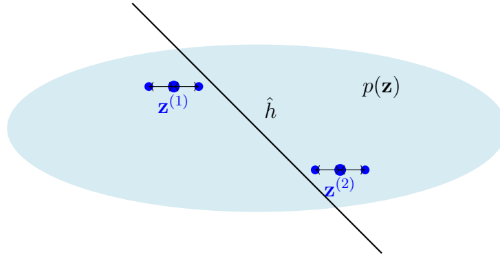
Fig. 90. Two data points \mathbf{z}^{(1)}, \mathbf{z}^{(2)} that are used as a training set to learn a hypothesis \hat{h} via ERM. We can evaluate \hat{h} outside \mathcal{D}^{(\text{train})} either by an i.i.d. assumption with some underlying probability distribution p(\mathbf{z}) or by perturbing the data points.
