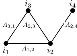
Fig. 89. An FL network with nodes \mathcal{V} = \{i_1, i_2, i_3, i_4\} representing four devices of an federated learning system (FL system).
