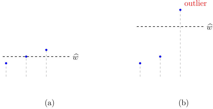
Fig. 109. For a linear model with d = 1 and using the trivial feature x = 1 for any data point, linear regression reduces to computing the average \hat{w} = (1/m) \sum_{r=1}^m y^{(r)} . (a) A clean training set and resulting parameter (given by the average). (b) A perturbed dataset (including an outlier) and the resulting parameter.
