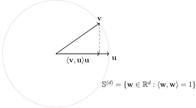
Fig. 34. For two unit-norm vectors \mathbf{u}, \mathbf{v} \in \mathbb{S}^{(d)} \subseteq \mathbb{R}^d the inner product \langle \mathbf{u}, \mathbf{v} \rangle is the expansion coefficient for the projection of \mathbf{v} onto the subspace \{c\mathbf{u} : c \in \mathbb{R}\} spanned by \mathbf{u} . The absolute value |\langle \mathbf{u}, \mathbf{v} \rangle| measures the norm of this projection.
