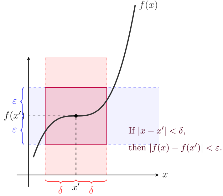
Fig. 9. The function f(x) = 0.3(x - 2)^3 + 2.5 is continuous at every x' .
