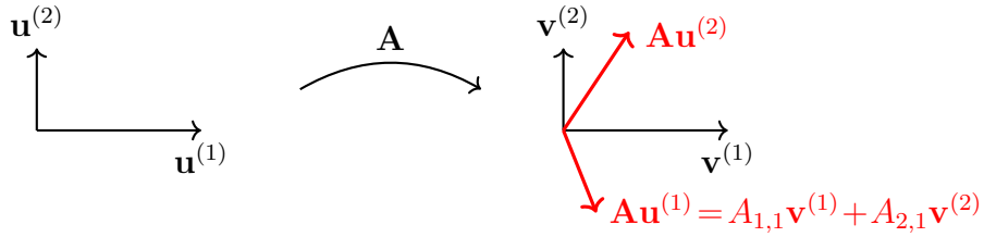
Fig. 41. A matrix \mathbf{A} defines a linear map between two vector spaces.
