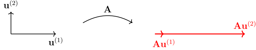
Fig. 55. Example of a rank-deficient matrix \mathbf{A} \in \mathbb{R}^{2 \times 2} .
