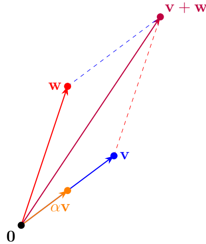
Fig. 62. A vector space \mathcal{V} is a collection of vectors such that scaling and adding them always yields another vector in \mathcal{V} .
