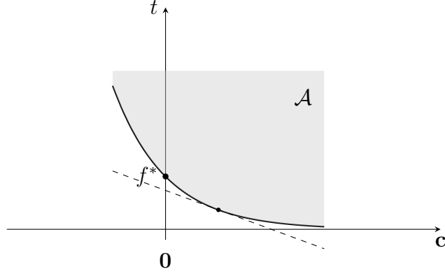
Fig. 13. A convex optimization problem (1) can be represented by a set \mathcal{A} that consists of objective values t and constraint values \mathbf{c} = (c_1, \dots, c_d)^T that are achievable, i.e., f(\mathbf{w}) \leq t, g_1(\mathbf{w}) \leq c_1, \dots, g_k(\mathbf{w}) \leq c_k for some \mathbf{w} \in \mathbb{R}^d . The optimal value f^* of the optimization problem is the smallest t for which (\mathbf{0}, t) \in \mathcal{A} .
