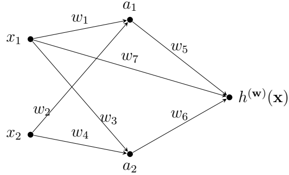
Fig. 65. An ANN can be represented as a weighted DAG with nodes that correspond to neurons or features of a data point. Features can be viewed as trivial neurons without input and with a fixed output given by the feature value. The weighted directed edges indicate how neuron outputs are used as inputs to other neurons. The edge weights are tunable model parameters and are used to scale the inputs to the neurons. The output of some neurons is used as the prediction h^{(\mathbf{w})}(\mathbf{x}) .
