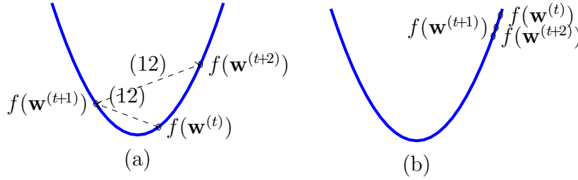
Fig. 104. Effect of using an inadequate learning rate \eta in the gradient step (12). (a) If \eta is too large, the gradient steps can “overshoot” such that the iterates \mathbf{w}^{(t)} diverge away from the optimum, i.e., f(\mathbf{w}^{(t+1)}) > f(\mathbf{w}^{(t)}) . (b) If \eta is too small, the gradient steps make too little progress towards the optimum within the available number of iterations (due to limited computational budget).
