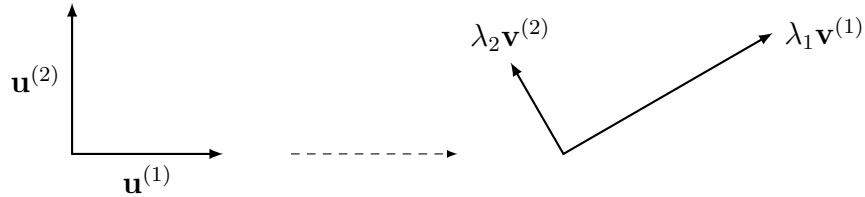
Fig. 57. Orthonormal matrices \mathbf{V} and \mathbf{U} .
