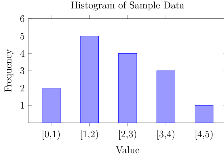
Fig. 94. A histogram consists of the fractions of data points that fall within different value ranges (i.e., bins). Each bar height shows the count of samples in the corresponding interval.
