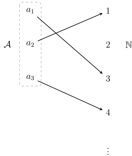
Fig. 14. An injective function that maps the elements of a finite set \mathcal{A} to the natural numbers \mathbb{N} , which implies that \mathcal{A} is countable.
