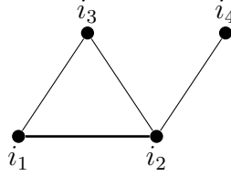
Fig. 32. A simple undirected graph with four nodes \mathcal{V} = \{i_1, i_2, i_3, i_4\} and four edges \mathcal{E} = \{\{i_1, i_2\}, \{i_2, i_3\}, \{i_3, i_1\}, \{i_2, i_4\}\} .
