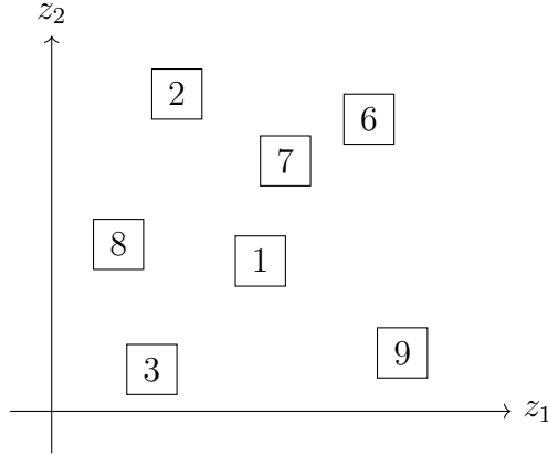
Fig. 80. Example of dimensionality reduction: High-dimensional image data (e.g., high-resolution images of handwritten digits) embedded into 2-D using learned features (z_1, z_2) and visualized in a scatterplot.
