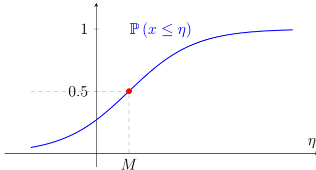
Fig. 43. The median of a real-valued RV is any number M that partitions \mathbb{R} into two rays with equal probability.
