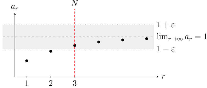
Fig. 11. A real-valued sequence (a_r)_{r \in \mathbb{N}} converging to the limit a^* = 1 .
