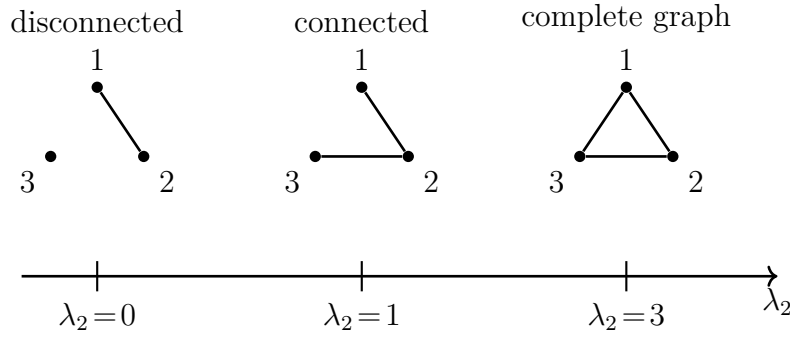
Fig. 1. Three examples of undirected graphs.
