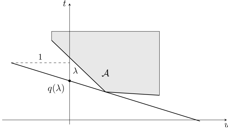
Fig. 37. The Lagrange dual function q(\lambda) , for a given \lambda \geq 0 , is the vertical intercept of a supporting hyperplane with normal vector (\lambda, 1) to the set \mathcal{A} = \{(u, t) : f(\mathbf{x}) \leq t, g_1(\mathbf{x}) \leq u \text{ for some } \mathbf{x} \in \mathbb{R}^d\} [23, Sec. 5.3].
