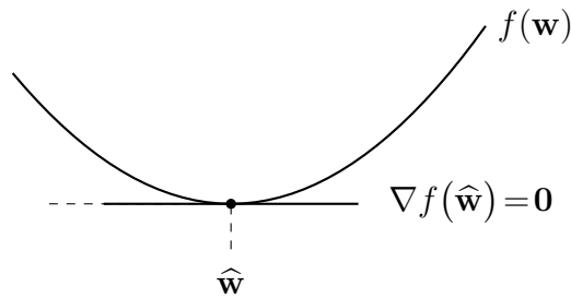
Fig. 142. A vector \hat{\mathbf{w}} solves the optimization problem if the gradient satisfies \nabla f(\hat{\mathbf{w}}) = \mathbf{0} .
