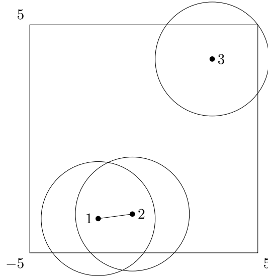
Fig. 54. Illustration of an RGG with \mathcal{X} = [-5, 5] \times [-5, 5] \subset \mathbb{R}^2 and radius r = 2.5 (with respect to the Euclidean distance), where nodes 1 and 2 (corresponding to (-2.0, -3.5)^T and (-0.5, -3.3)^T , within radius r = 2.5 ) are connected, while node 3 (corresponding to (3.0, 3.5)^T ) has no other node within that distance.
