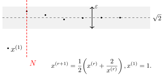
Fig. 5. A Cauchy sequence (x^{(r)})_{r \in \mathbb{N}} in the metric space (\mathbb{Q}, |\cdot|) . This sequence is generated by a fixed-point iteration used to approximate \sqrt{2} . For all r \geq N , the sequence elements lie within a band of width \varepsilon . Note that the sequence does not converge in \mathbb{Q} , since \sqrt{2} \notin \mathbb{Q} [2, Example 1.1].
