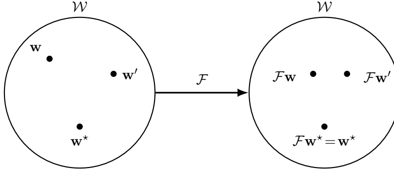
Fig. 2. A contractive operator \mathcal{F} : \mathcal{W} \rightarrow \mathcal{W} has a unique fixed point \mathbf{w}^* with \mathcal{F}\mathbf{w}^* = \mathbf{w}^* .
