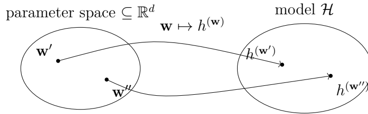
Fig. 117. The model parameters \mathbf{w} select a well-defined hypothesis h(\mathbf{w}) out of the model \mathcal{H} .
