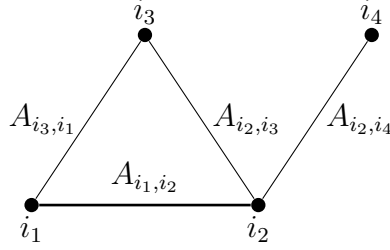
Fig. 63. A weighted graph with four nodes \mathcal{V} = \{i_1, i_2, i_3, i_4\} and four edges \mathcal{E} = \{\{i_1, i_2\}, \{i_2, i_3\}, \{i_3, i_1\}, \{i_2, i_4\}\} . Each edge is assigned a weight.
