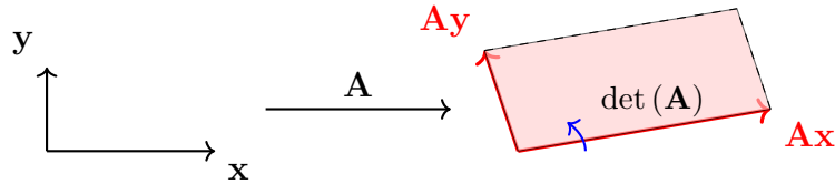
Fig. 17. We can interpret a square matrix \mathbf{A} as a linear transformation of \mathbb{R}^d into itself. The determinant \det(\mathbf{A}) characterizes how this transformation alters an oriented volume.
