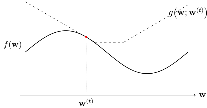
Fig. 39. The construction of model parameters based on the iterative MM method.
