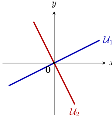
Fig. 59. Any \mathbf{x} \in \mathbb{R}^2 defines a subspace of \mathcal{U}_{\mathbf{x}} \subset \mathbb{R}^2 by \mathcal{U}_{\mathbf{x}} = \{\lambda \cdot \mathbf{x} : \lambda \in \mathbb{R}\} \subset \mathbb{R}^2 . For \mathbf{x} \neq \mathbf{0} , this corresponds to straight lines through the origin (illustrated by \mathcal{U}_1 and \mathcal{U}_2 ), for the zero vector \mathbf{x} = \mathbf{0} this leads to the trivial subspace \{\mathbf{0}\} just containing the zero vector.
