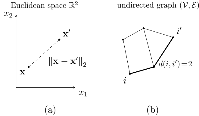
Fig. 45. Examples of metric spaces. (a) Euclidean space \mathbb{R}^2 with the Euclidean distance as a metric. (b) Undirected graph (\mathcal{V}, \mathcal{E}) with the shortest-path distance as a metric.
