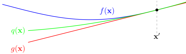
Fig. 33. A function f(\mathbf{x}) that is sufficiently smooth at a point \mathbf{x}' can be locally approximated by a quadratic function q(\mathbf{x}) , which provides a more accurate approximation compared to a linear function g(\mathbf{x}) .
