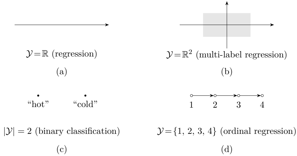
Fig. 102. Examples of label spaces and the corresponding types of ML. (a) Regression. (b) Multi-label regression. (c) Binary classification. (d) Ordinal regression.
