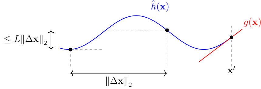
Fig. 108. A trained model \hat{h}(\mathbf{x}) that is differentiable at a point \mathbf{x}' can be locally approximated by a linear map g \in \mathcal{H}^{(d)} . This local approximation is determined by the gradient \nabla \hat{h}(\mathbf{x}') .
