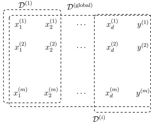
Fig. 139. VFL uses local datasets that are derived from the data points of a common global dataset. The local datasets differ in the choice of features used to characterize the data points.
