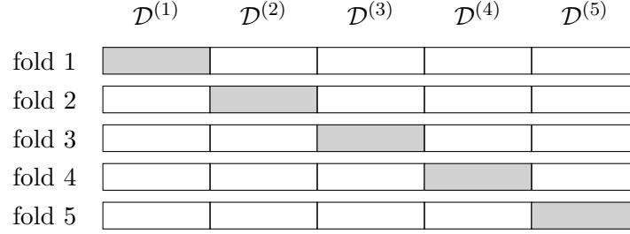
Fig. 99. In k -fold CV, the available dataset \mathcal{D} is evenly divided into k folds \mathcal{D}^{(1)}, \dots, \mathcal{D}^{(k)} . Each fold is used once as a validation set, while the remaining k - 1 folds form the training set.
