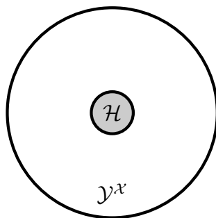
Fig. 96. The hypothesis space \mathcal{H} of an ML method is a (typically very small) subset of the (typically very large) set \mathcal{Y}^{\mathcal{X}} of all possible maps from the feature space \mathcal{X} into the label space \mathcal{Y} .
