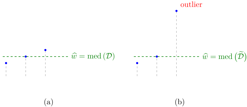
Fig. 106. For the simple parametric model h^{(w)}(\mathbf{x}) = w , ERM with absolute error loss amounts to computing the median. (a) Original dataset \mathcal{D} . (b) Noisy dataset \tilde{\mathcal{D}} including an outlier.
