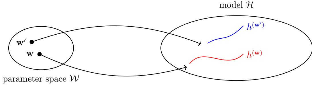
Fig. 122. The parameter space \mathcal{W} of an ML model \mathcal{H} consists of all feasible choices for the model parameters. Each choice \mathbf{w} for the model parameters selects a hypothesis map h^{(\mathbf{w})} \in \mathcal{H} .
