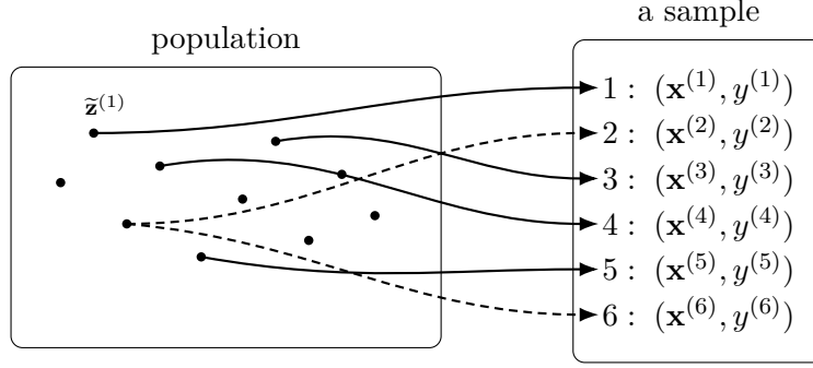
Fig. 56. A sample viewed as a finite sequence. Each element of this sample consists of the feature vector and the label of a data point from an underlying population. The same data point may occur more than once in the sample.
