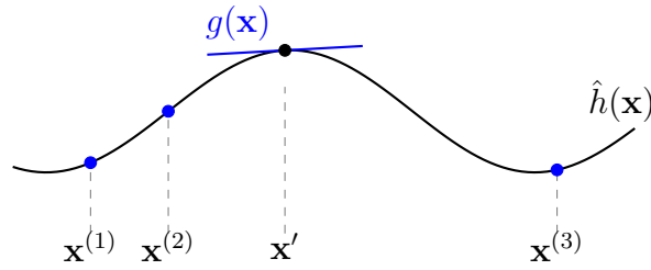
Fig. 85. A trained model \hat{h}(\mathbf{x}) can be explained locally at some point \mathbf{x}' by a linear approximation g(\mathbf{x}) . For a differentiable \hat{h}(\mathbf{x}) , this approximation is determined by the gradient \nabla \hat{h}(\mathbf{x}') . Another form of explanation could be the function values \hat{h}(\mathbf{x}^{(r)}) for r = 1, 2, 3 .
