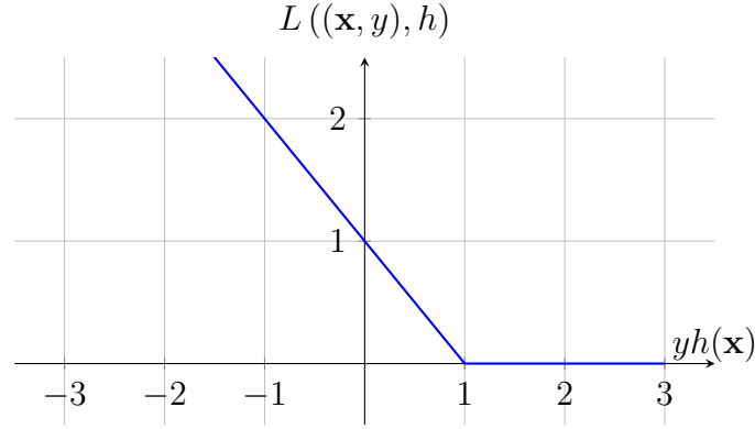
Fig. 93. The hinge loss incurred by the prediction h(\mathbf{x}) \in \mathbb{R} for a data point with label y \in \{-1, 1\} . A regularized variant of the hinge loss is used by the support vector machine (SVM) [142].
