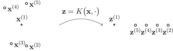
Fig. 101. Five data points characterized by feature vectors \mathbf{x}^{(r)} and labels y^{(r)} \in \{\circ, \square\} , for r = 1, \dots, 5 . With these feature vectors, there is no way to separate the two classes by a straight line (representing the decision boundary of a linear classifier). In contrast, the transformed feature vectors \mathbf{z}^{(r)} = K(\mathbf{x}^{(r)}, \cdot) allow us to separate the data points using a linear classifier.
