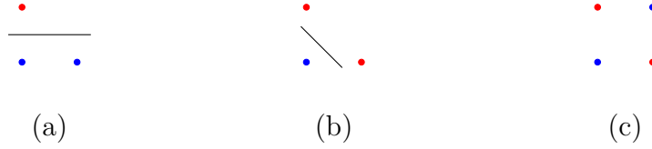
Fig. 138. Illustration of the VC dimension for a linear model \mathcal{H}^{(2)} that is used to learn a linear classifier in the feature space \mathbb{R}^2 .
