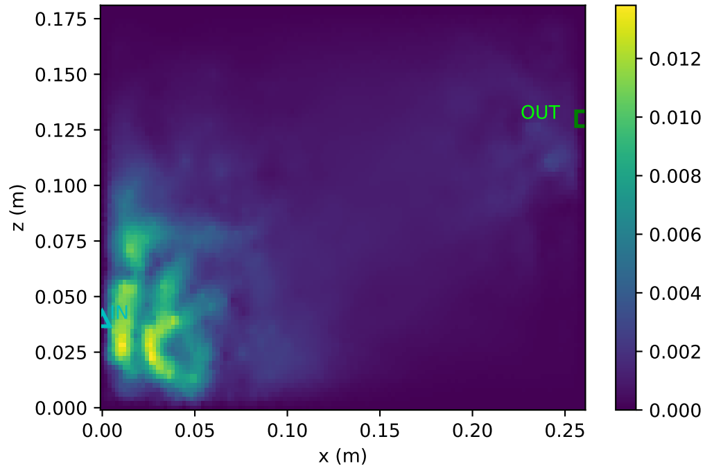
|u| (m/s) — plano y = Ly/2
