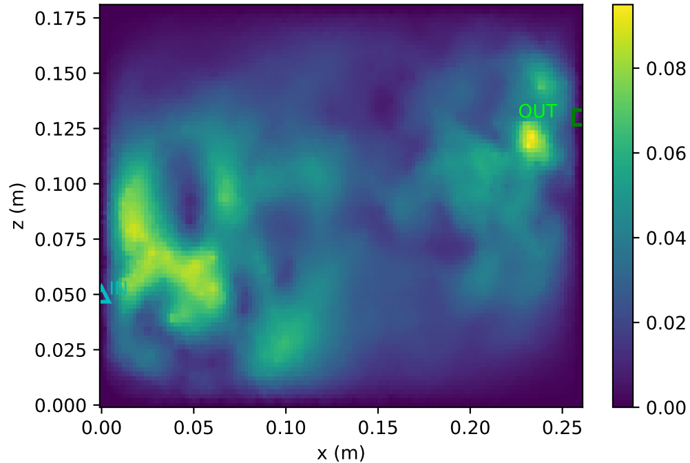
|u| (m/s) — plano y = Ly/2
