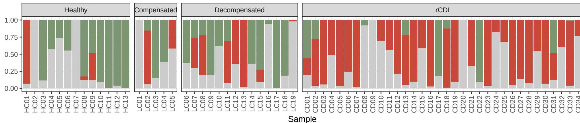
=50% completeness, &lt;5% Contamination
