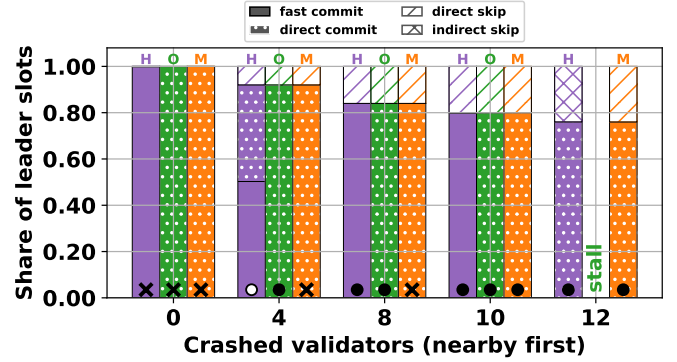
Fig. 10. Decision rule of every leader slot vs. crashed validators, n = 50 , 10k tx/s (H: Hydrozoan, O: Orcaella, M: Mysticeti). Foot symbol: no quorum needs Tokyo (X), only the fast quorum does (O), the round quorum does (●).
