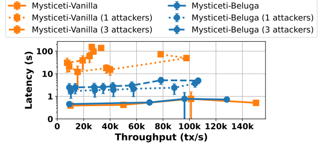
Figure 6: Throughput–latency of Mysticeti with Beluga vs. the baseline push-pull synchronizer under the pull induction attack. WAN, 10 validators, 0/1/3 faults, 512B transactions; log-scale latency.
