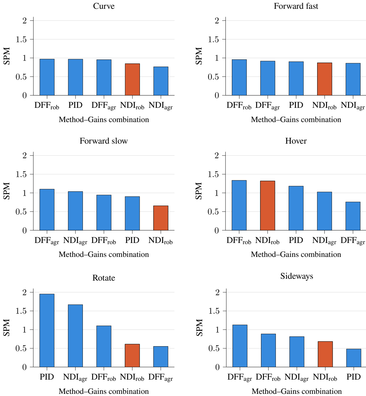
Figure 5.12.: Comparison of the Scenario Performance Metric across selected controller/gain combinations for each flight scenario, sorted from highest to lowest. The orange bar highlights the NDI controller with Robust gains.
