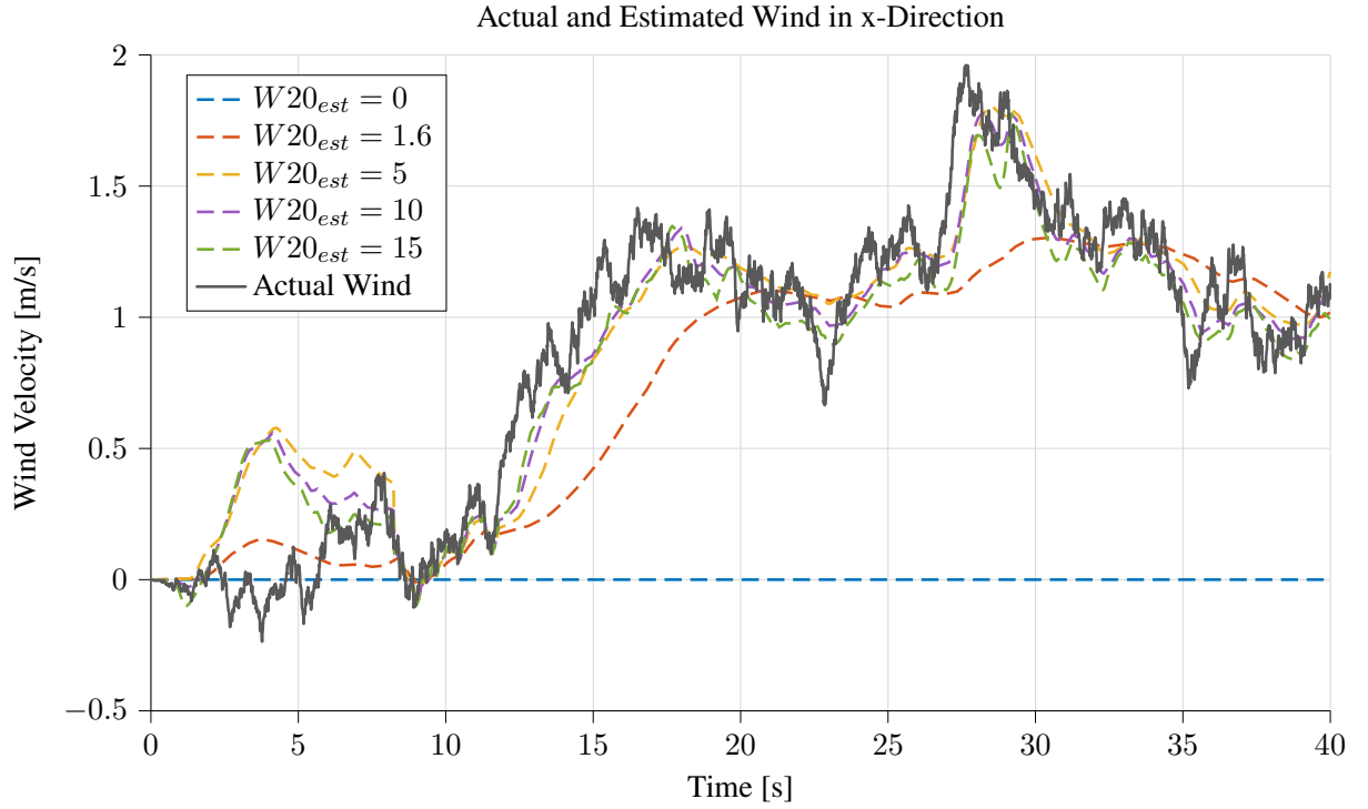
Figure 5.2.: Comparison of wind estimation performance for different assumed reference wind speeds W_{20,ass} and W_{20,true} = 5 .
