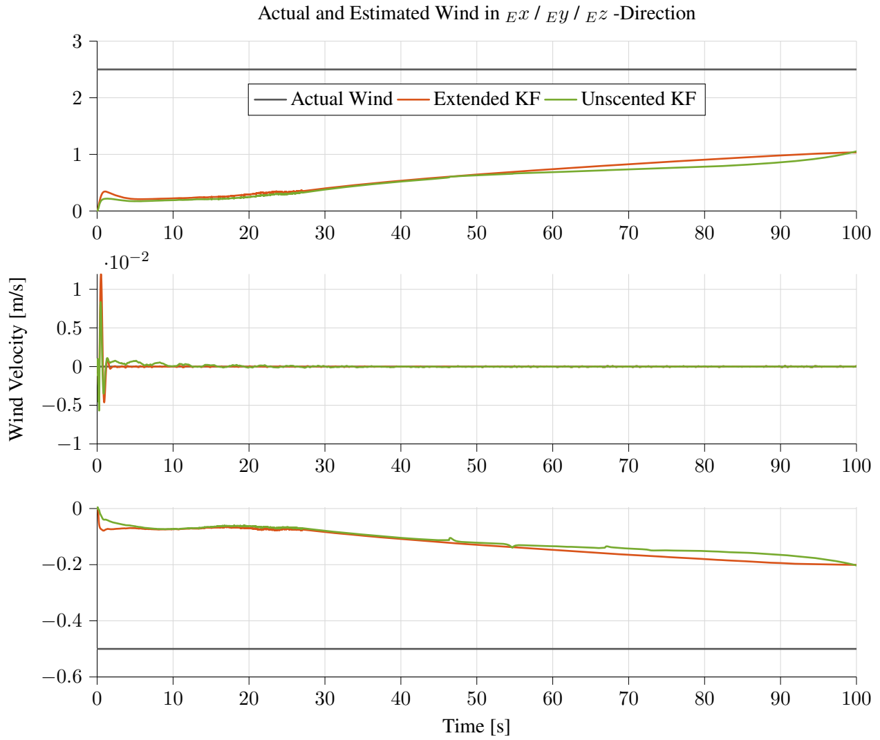
Figure 5.8.: Actual and estimated wind for hover flight scenario, constant wind component \mathbf{v}_{W,\text{const}} = [2.5 \ 0 \ -0.5] \text{ m/s} and W_{20,\text{true}} = 0 \text{ m/s} . Process noise is disabled for visualization purposes to highlight the convergence behavior of the wind estimate.
