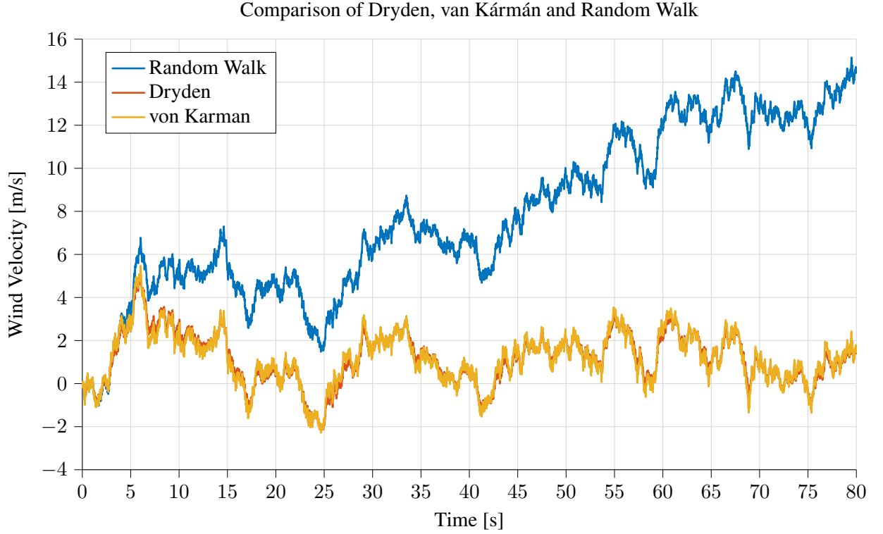
Figure 2.2.: Comparison of wind turbulence created by the random walk, von Kármán and Dryden model for identical white noise input.
