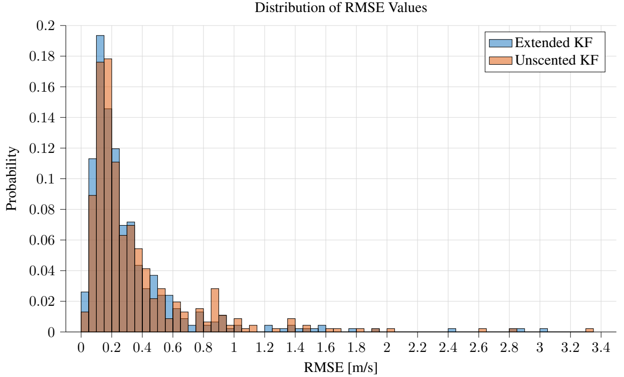
Figure 5.4.: Distribution of the per-run wind estimation RMSE for the EKF and UKF across the investigated test suite.
