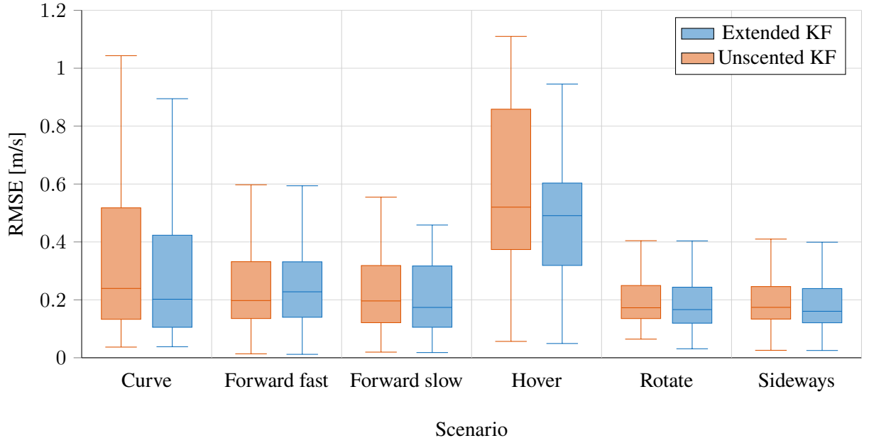
Figure 5.6.: Average wind estimation RMSE by scenario for Unscented KF and Extended KF. Boxes show the interquartile range (Q1–Q3) with the median line; whiskers extend to the most extreme point within 1.5 \times \text{IQR} . Outlier points beyond the whiskers are omitted.
