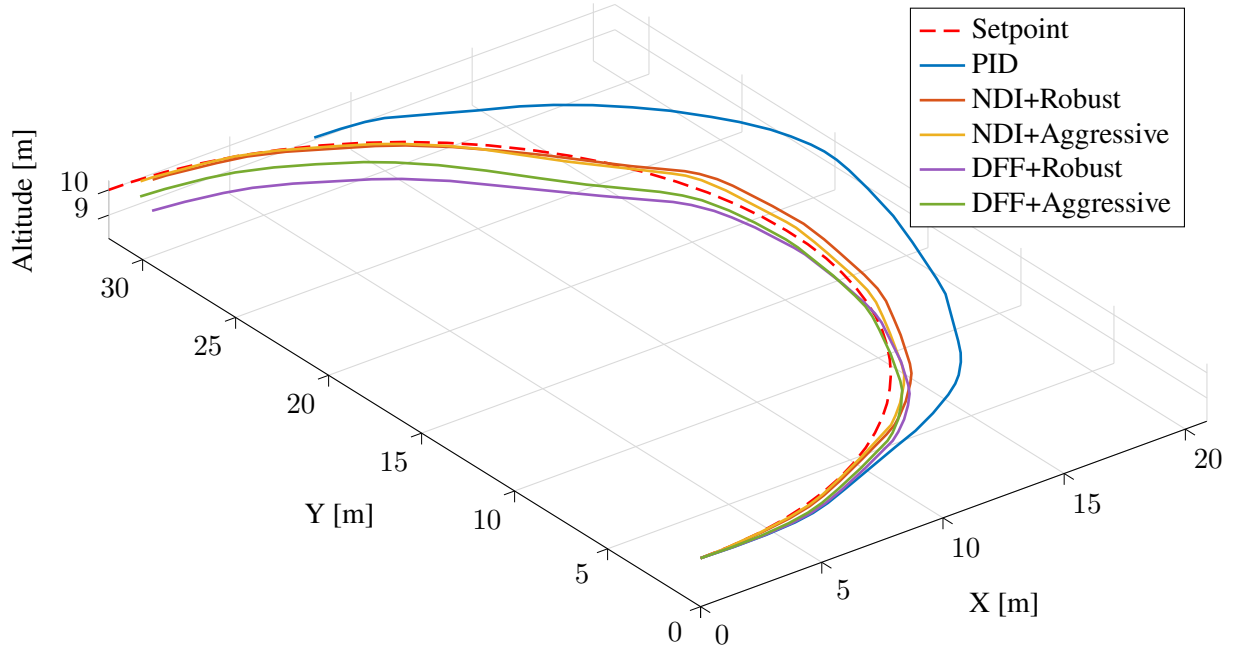
Figure 5.11.: Comparison of the trajectories for the PID baseline and the DFF and NDI compensation approaches with Robust and Aggressive gain settings for a representative Curve scenario test run.
