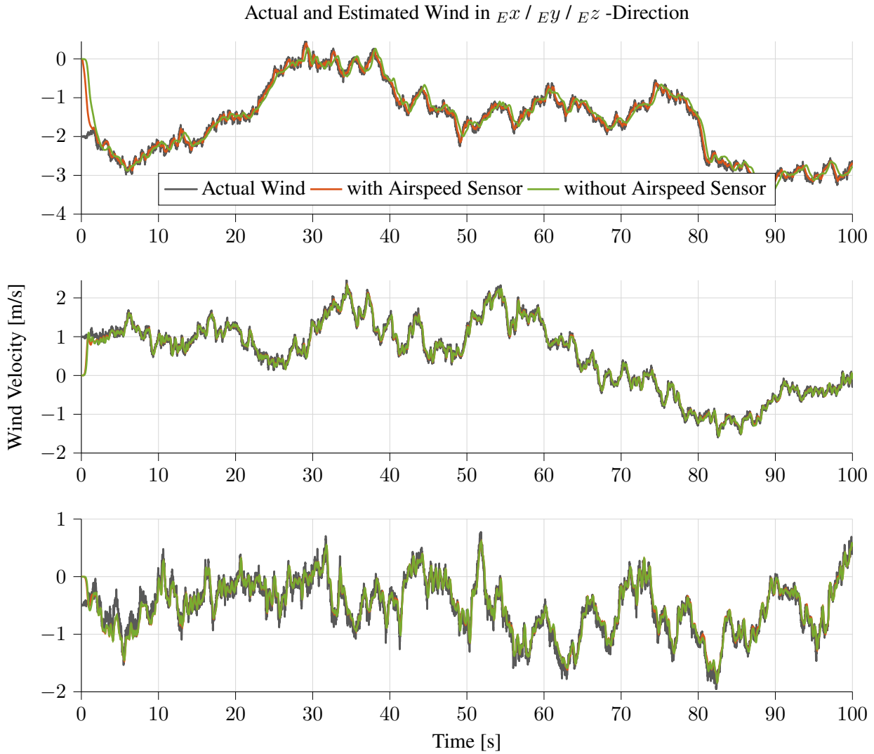
Figure 5.9.: Comparison of EKF wind estimation with and without the 1D airspeed measurement for the Forward fast scenario with \mathbf{v}_{W,\text{const}} = [-2 \ 1 \ -0.5] \text{ m/s} and W_{20,\text{true}} = 5 \text{ m/s} .
