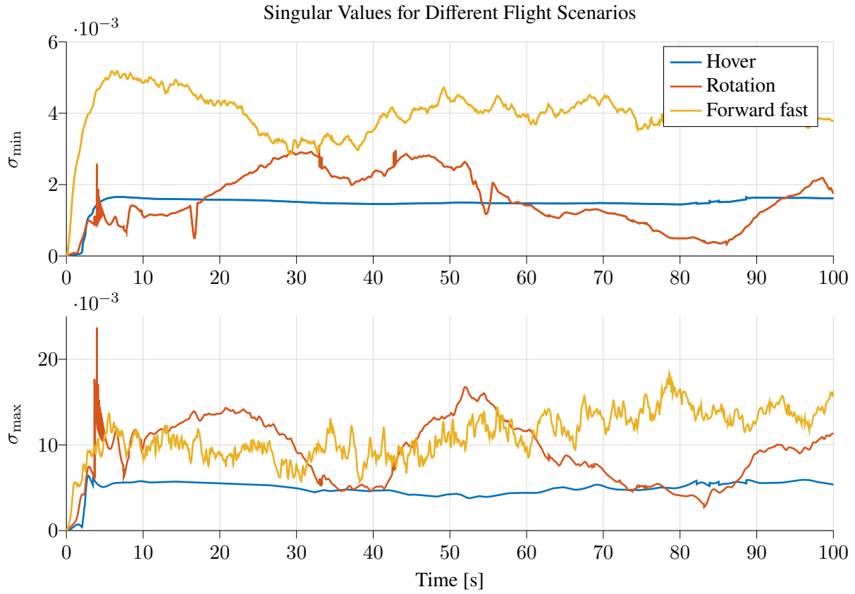
Figure 5.7.: Minimum (top) and maximum (bottom) singular values of \mathbf{F}_{v_W} over time for Hover, Forward fast, and Rotation, with constant wind component \mathbf{v}_{W,\text{const}} = [-2 \ 0 \ -0.5] \text{ m/s} and reference wind speed W_{20,\text{true}} = 5 \text{ m/s} .
