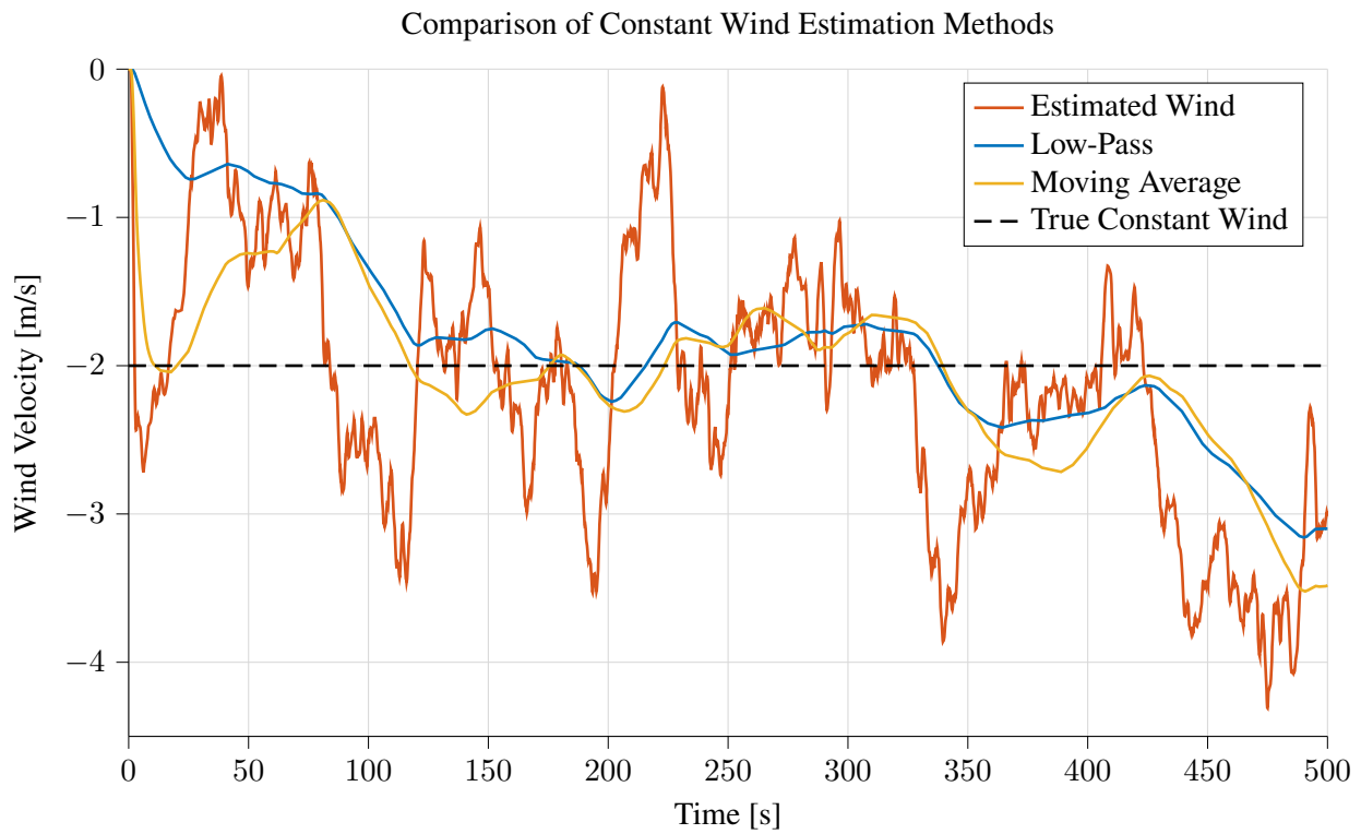
Figure 5.10.: Comparison of the true constant wind component with estimates obtained by applying low-pass filtering and a moving average to the wind estimate from the Kalman filter, over a 500 s flight.
