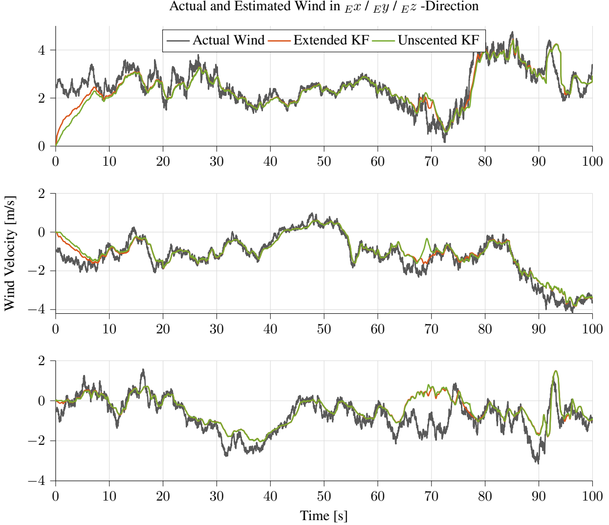
Figure 5.3.: Actual and estimated wind for Curve flight scenario, constant wind component \mathbf{v}_{W,\text{const}} = [2.5 \ -1 \ -0.5]\text{m/s} and reference wind speed W_{20,\text{true}} = 10\text{ m/s}
