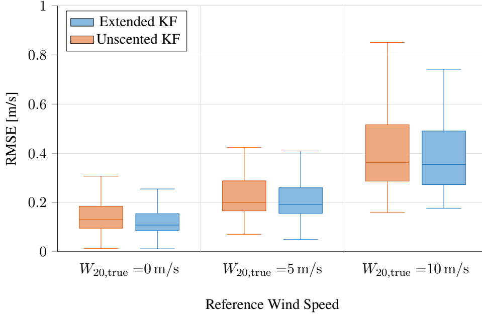
Figure 5.5.: Average wind estimation RMSE for different values of W_{20,true} , averaged over the six flight scenarios and 27 wind conditions. Boxes show the interquartile range (Q1–Q3) with the median line; whiskers extend to the most extreme point within 1.5 \times \text{IQR} . Outlier points beyond the whiskers are omitted.
