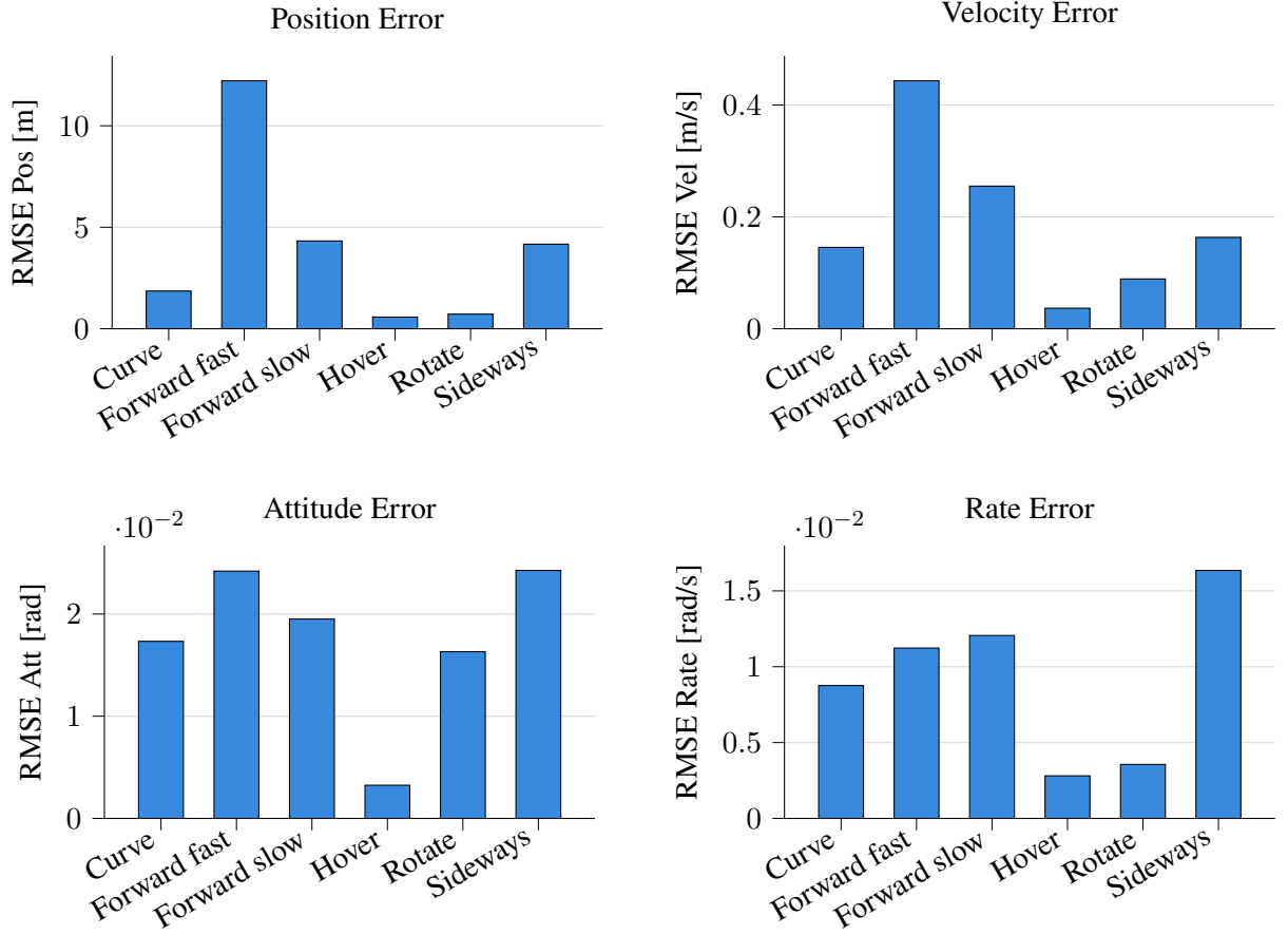
Figure 5.13.: Grouped Errors (position, velocity, attitude, and angular rate) for the NDI controller with Robust gains across all evaluated flight scenarios.
