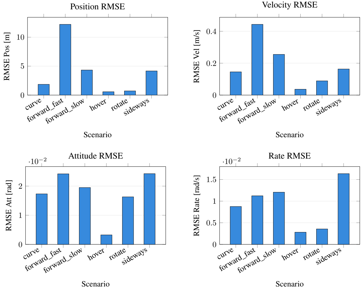
Figure 5.13.: Grouped RMSE (position, velocity, attitude, and angular rate) for the NDI controller with Robust gains across all evaluated flight scenarios.
