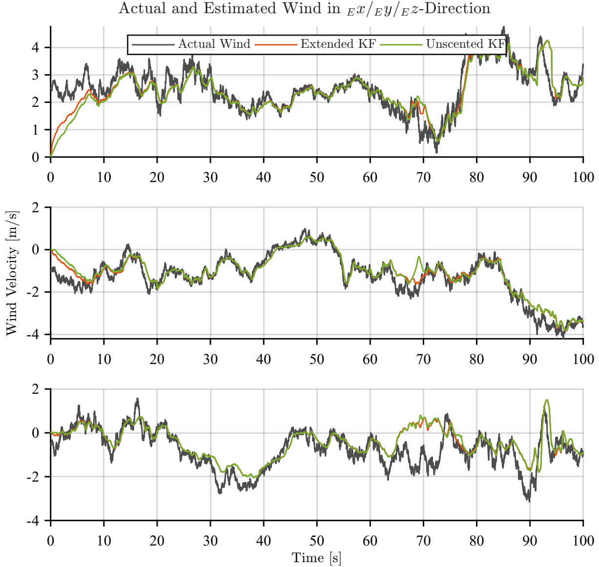
Figure 5.3.: Actual and estimated wind for curved flight scenario, constant wind component v_{W,\text{const}} = [2.5 - 1 - 0.5]\text{m/s} and W_{20,\text{true}} = 10
