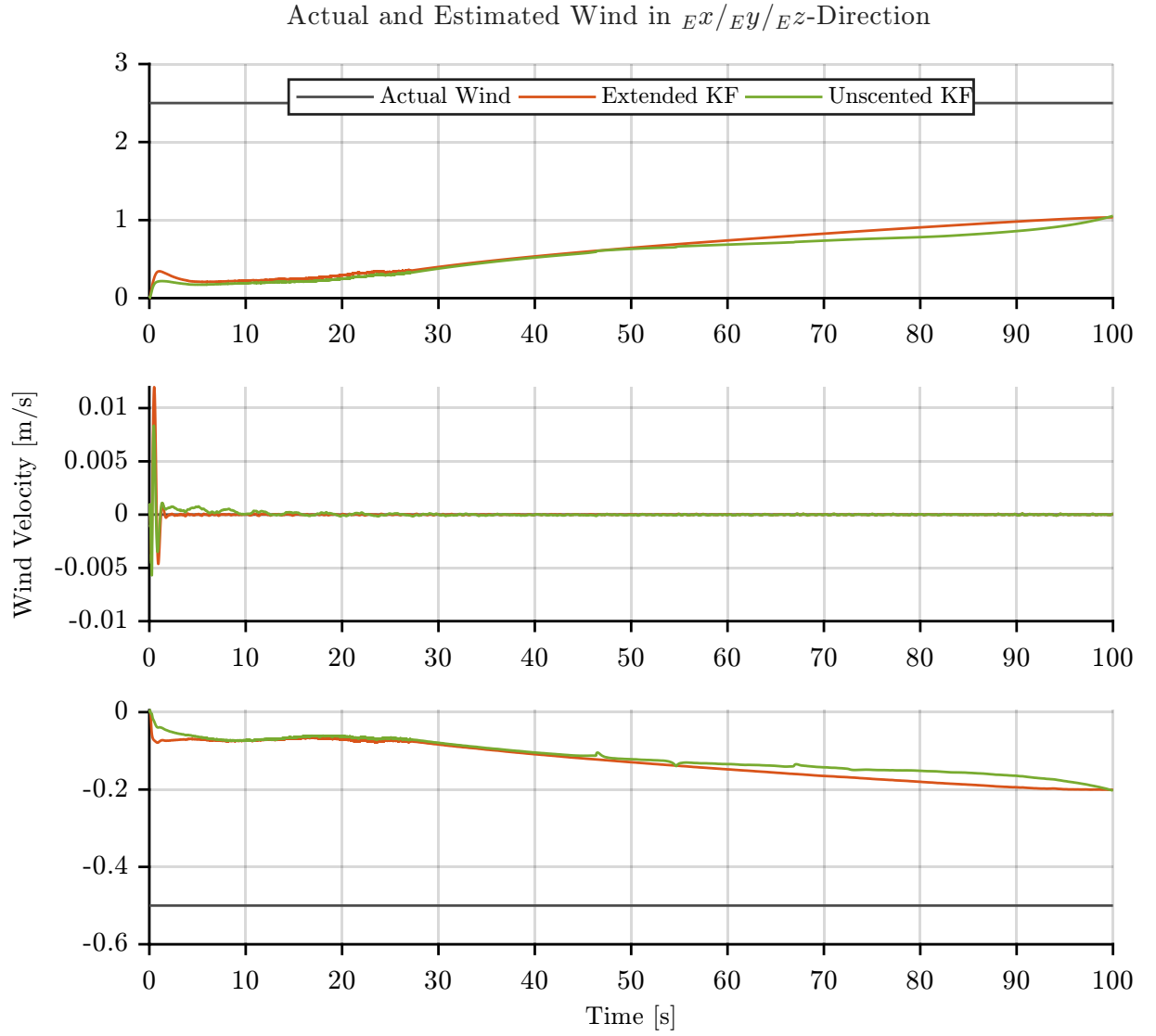
Figure 5.8.: CONSTANT WIND, No uncertainty. Process noise is disabled for visualization purposes to highlight the convergence behavior of the wind estimate.
