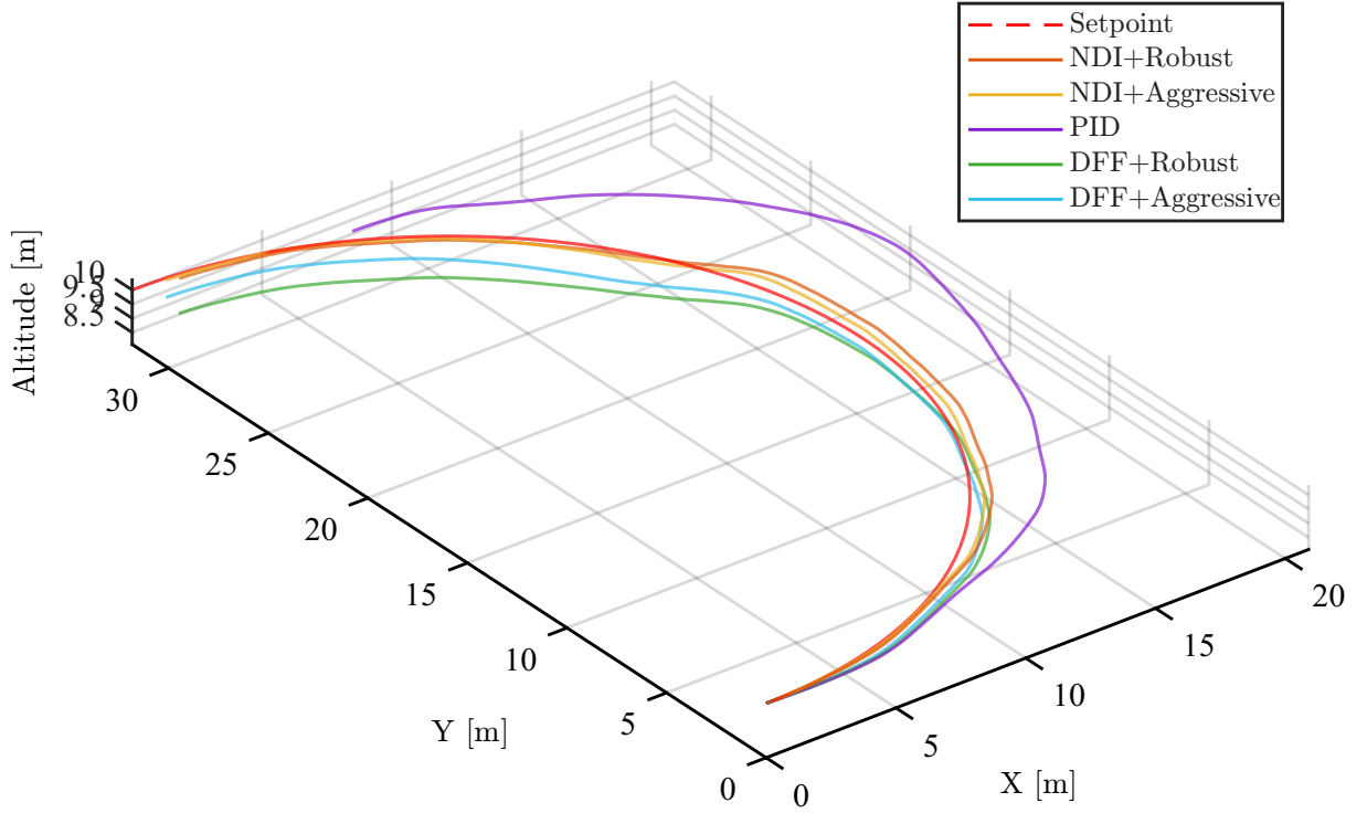
Figure 5.11.: Comparison of the trajectories for the PID baseline and the DFF and NDI compensation approaches with Robust and Aggressive gain settings for a representative Curve scenario test run.
