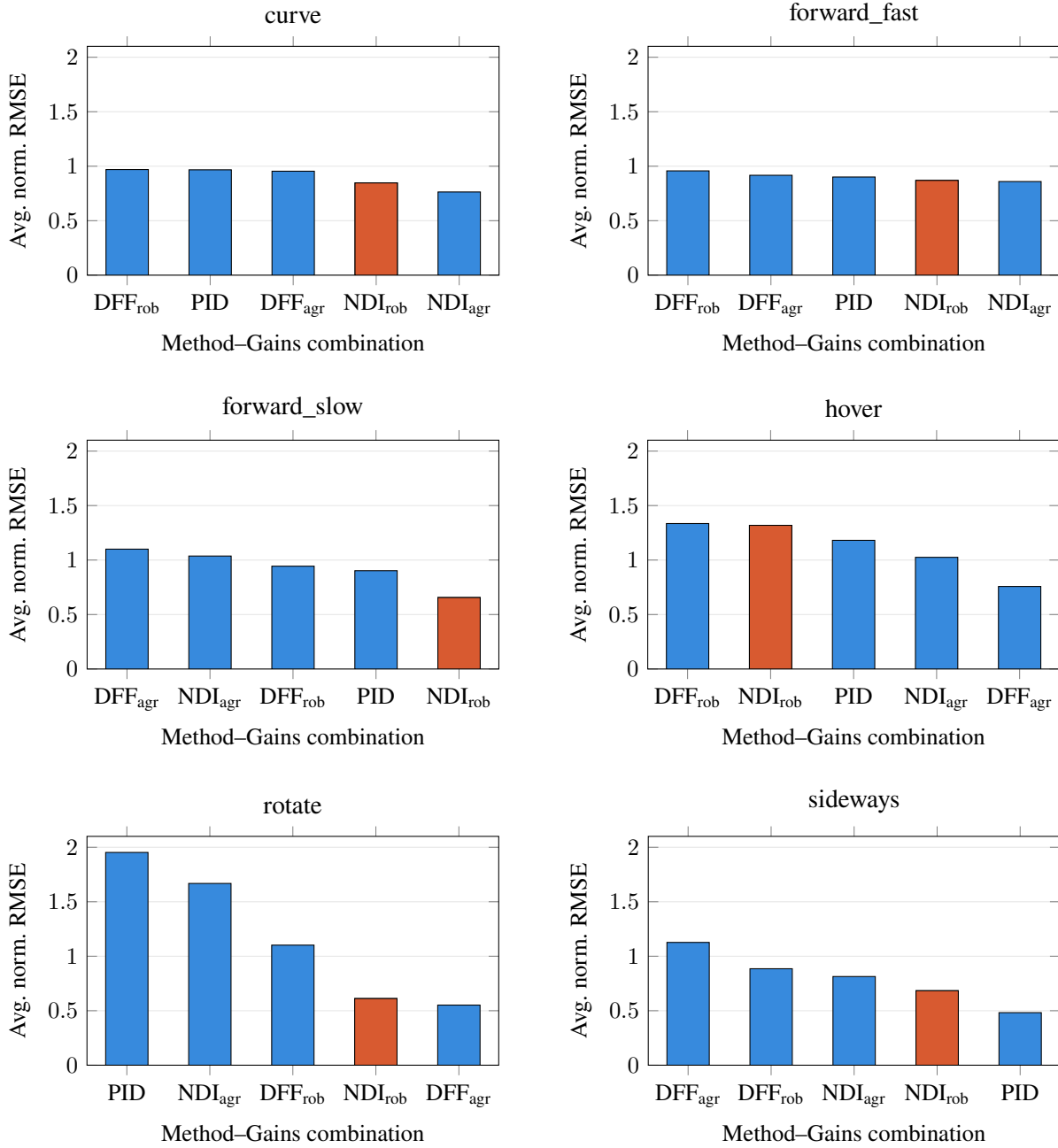
Figure 5.11.: Comparison of average normalized RMSE across selected controller/gain combinations for each flight scenario, sorted from highest to lowest. The orange bar highlights the NDI controller with Robust gains. The combinations NDI-Comp and DFF-Comp have been left out for better clarity.
