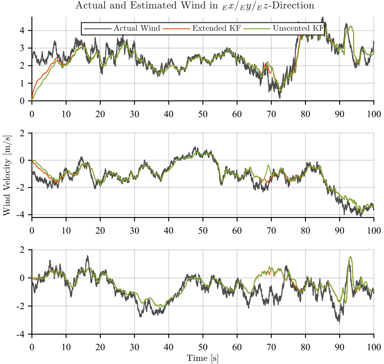
Figure 5.3.: Actual and estimated wind for curved flight scenario, constant wind component \mathbf{v}_{W,\text{const}} = [2.5 \ -1 \ -0.5] m/s and W_{20,\text{true}} = 10
