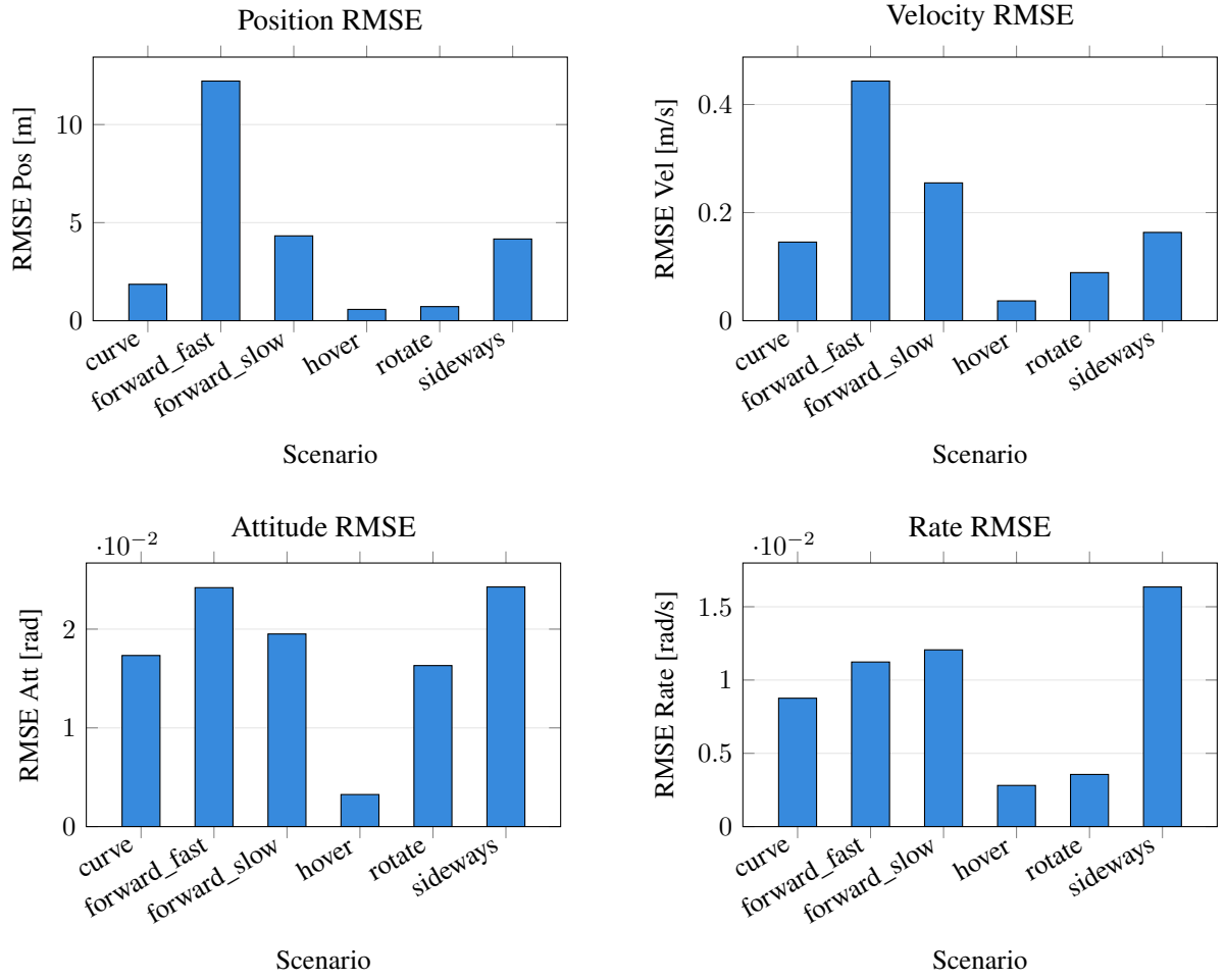
Figure 5.12.: Grouped RMSE (position, velocity, attitude, and angular rate) for the NDI controller with Robust gains across all evaluated flight scenarios.
