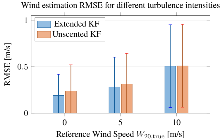
Figure 5.5.: Average wind estimation RMSE for different values of W_{20,\text{true}} , averaged over the six flight scenarios and 27 wind conditions. The line within indicates the standard deviation of the RMSE.
