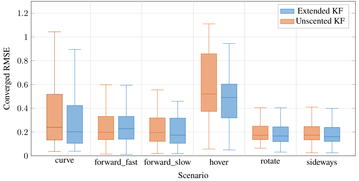
Figure 5.6.: Mean RMSE by scenario for Unscented KF and Extended KF. Boxes show the interquartile range (Q1–Q3) with the median line; whiskers extend to the most extreme point within 1.5 \times \text{IQR} . Outlier points beyond the whiskers are omitted.
