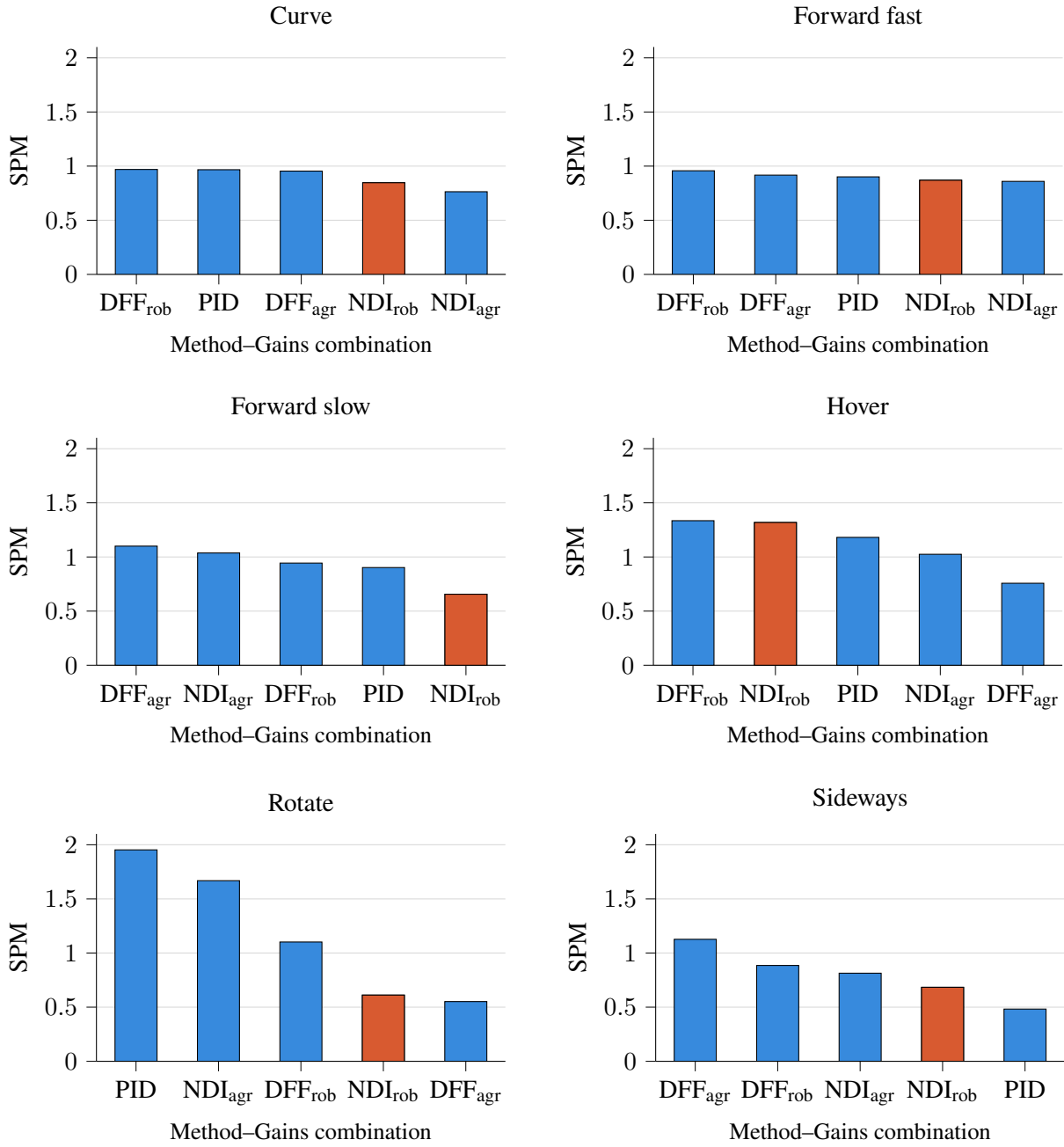
Figure 5.13.: Comparison of the Scenario Performance Metric across selected controller/gain combinations for each flight scenario, sorted from highest to lowest. The orange bar highlights the NDI controller with Robust gains.
