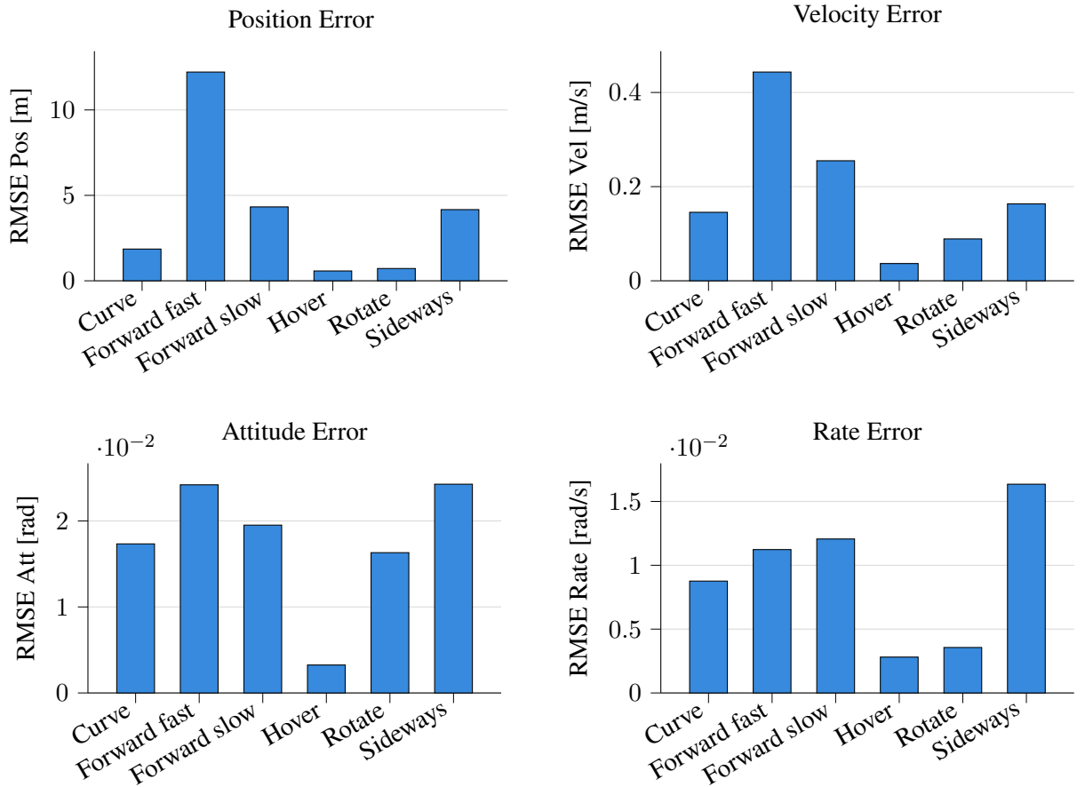
Figure 5.14.: Grouped Errors (position, velocity, attitude, and angular rate) for the NDI controller with Robust gains across all evaluated flight scenarios.
