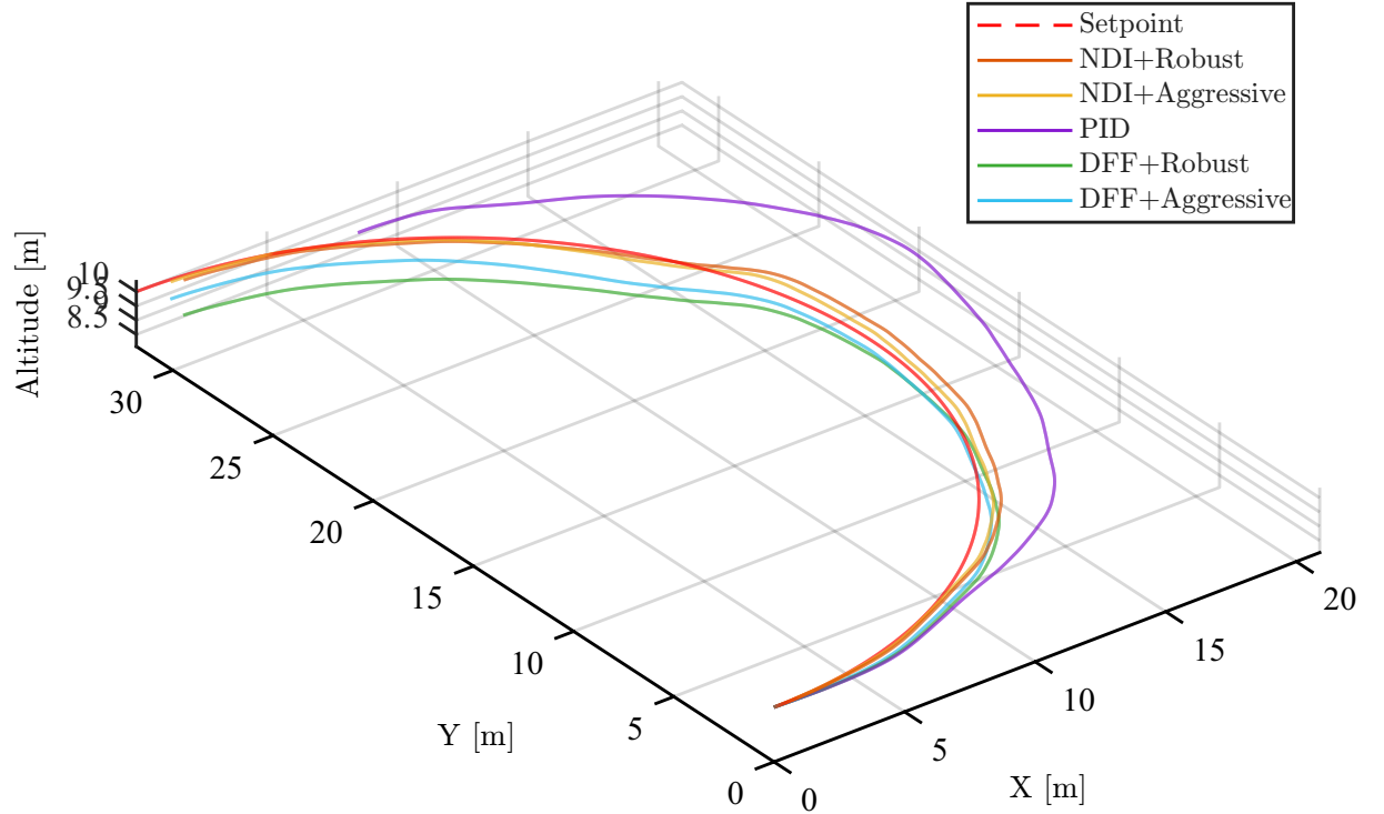
Figure 5.12.: Comparison of the trajectories for the PID baseline and the DFF and NDI compensation approaches with Robust and Aggressive gain settings for a representative Curve scenario test run.
