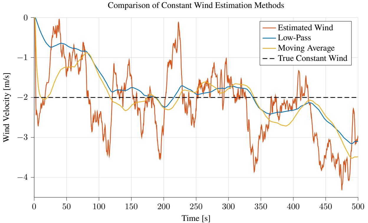
Figure 5.11.: Comparison of the true constant wind component with estimates obtained by applying low-pass filtering and a moving average to the wind estimate from the Kalman filter, over a 500 s flight.
