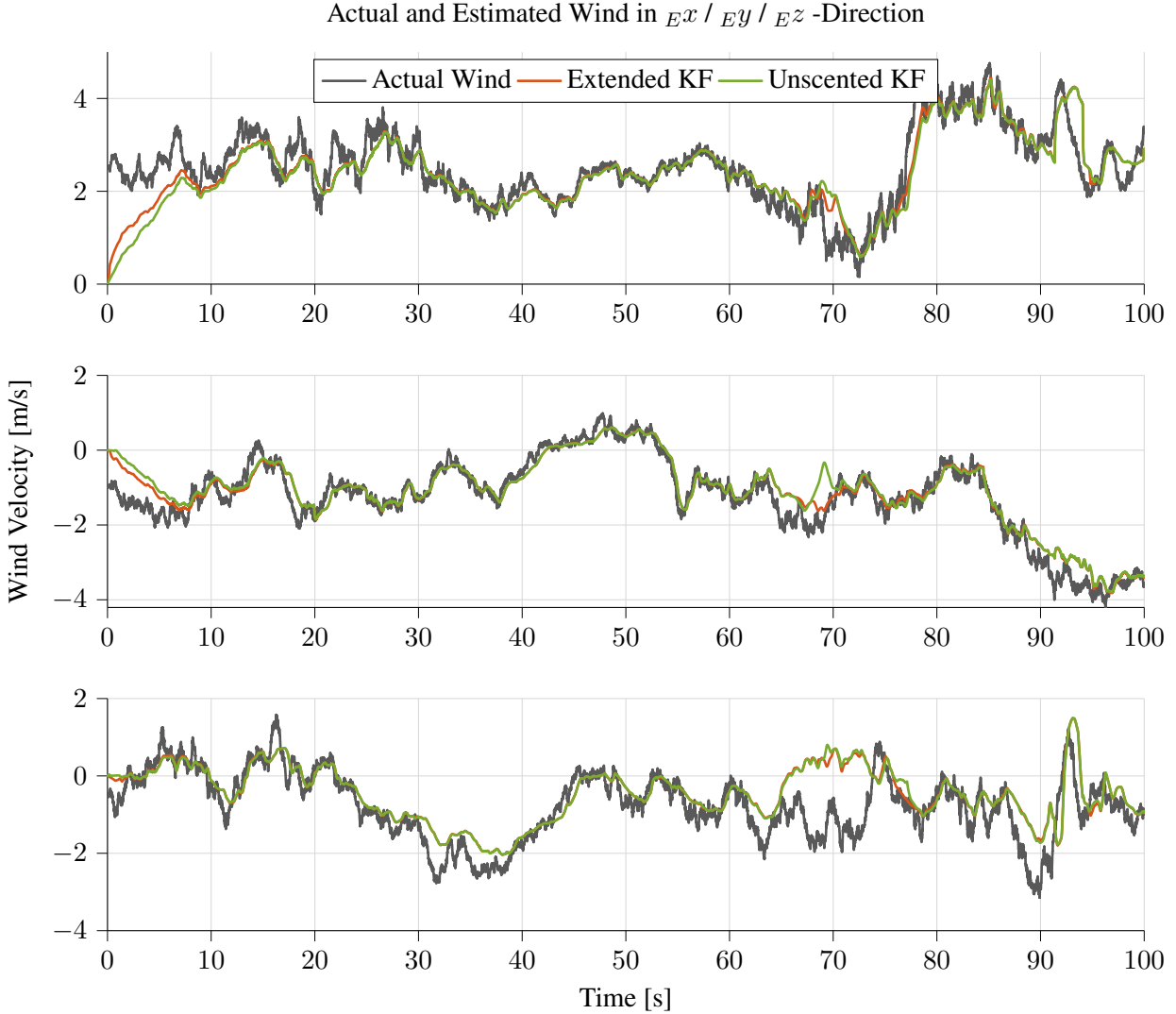
Figure 5.3.: Actual and estimated wind for Curve flight scenario, constant wind component \mathbf{v}_{W,\text{const}} = [2.5 - 1 - 0.5]\text{m/s} and reference wind speed W_{20,\text{true}} = 10\text{ m/s}
