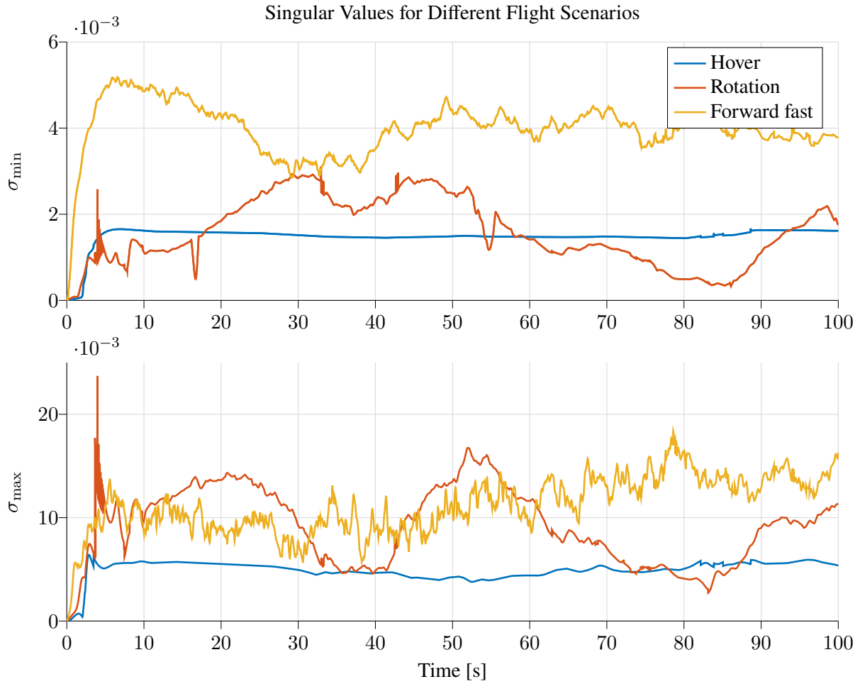
Figure 5.7.: Minimum (top) and maximum (bottom) singular values of F_{v_W} over time for Hover, Forward fast, and Rotation, with constant wind component v_{W,\text{const}} = [-2 \ 0 \ -0.5] \text{ m/s} and reference wind speed W_{20,\text{true}} = 5 \text{ m/s} .
