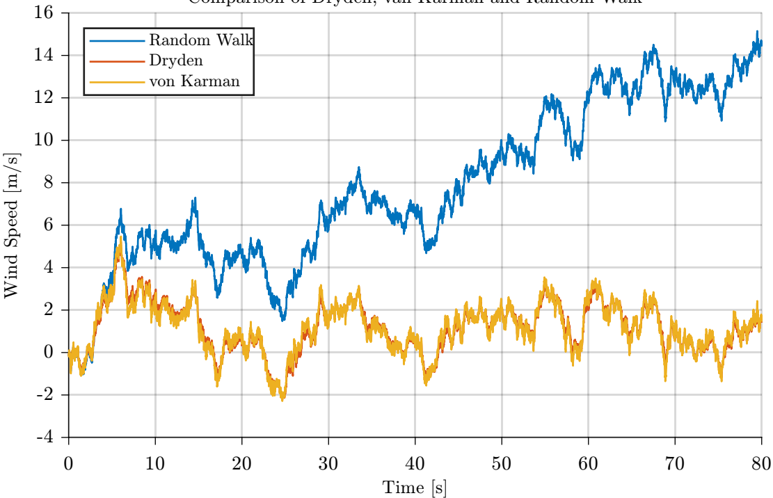
Comparison of Dryden, van Karman and Random Walk
