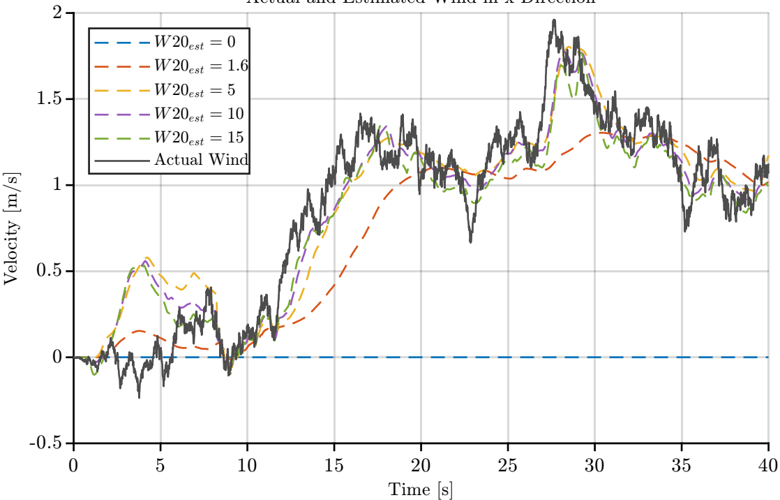
Actual and Estimated Wind in x-Direction
