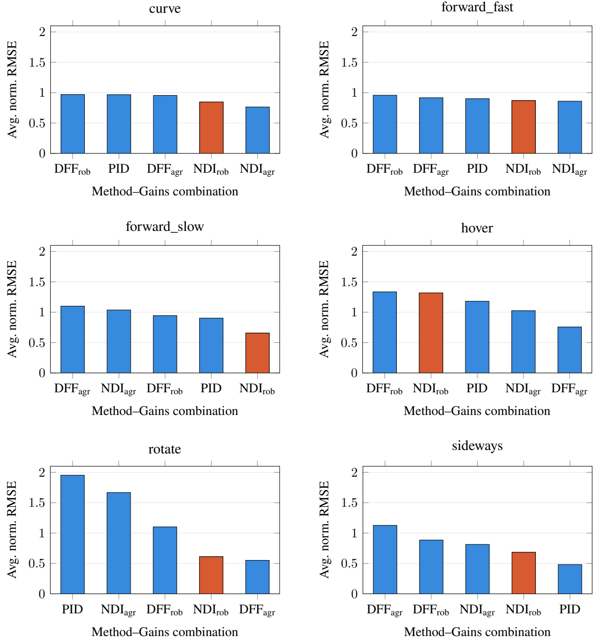
Figure 5.5.: Comparison of average normalized RMSE across selected controller/gain combinations for each flight scenario, sorted from highest to lowest. The orange bar highlights the NDI controller with Robust gains. The combinations NDI-Comp and DFF-Comp have been left out for better clarity.
