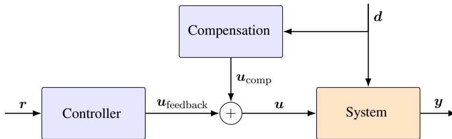
Figure 2.4.: Structure of a compensation-based control approach. Both the controller and the compensation module may utilize available system outputs. For clarity, the corresponding signal paths are omitted.
