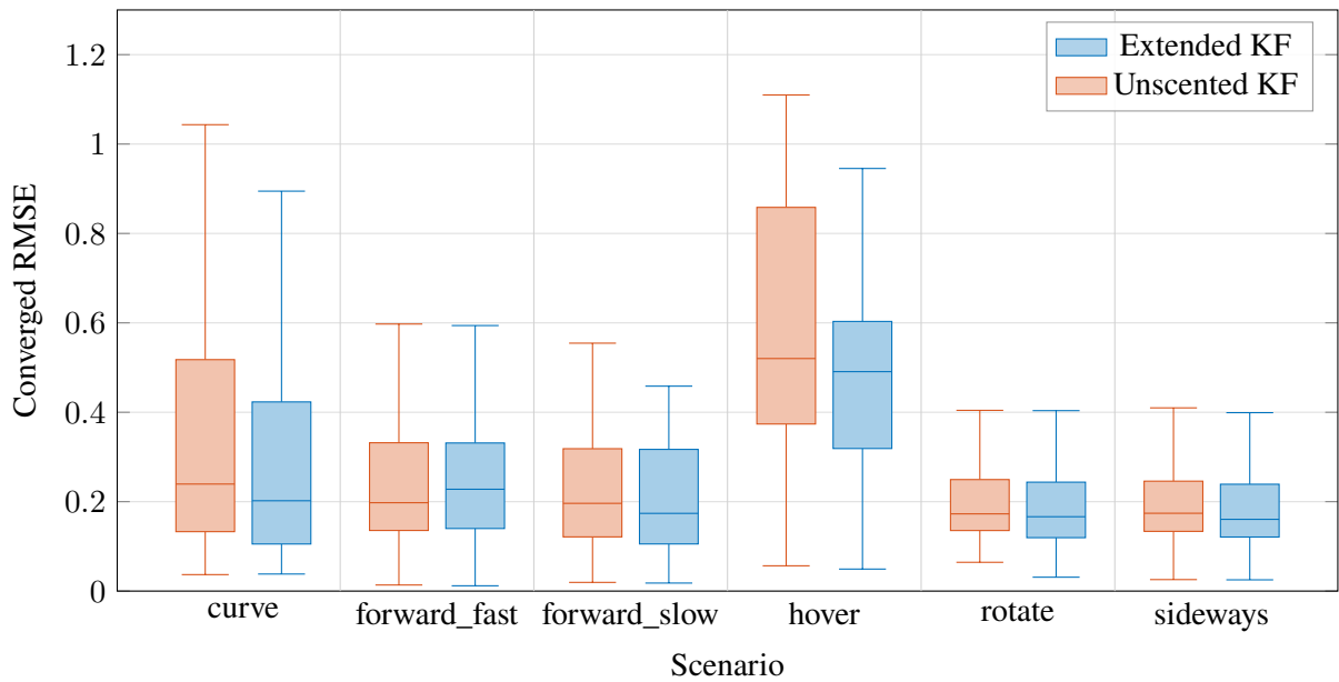
Figure 5.4.: Converged RMSE by scenario for Unscented KF and Extended KF. Boxes show the interquartile range (Q1–Q3) with the median line; whiskers extend to the most extreme point within 1.5 \times \text{IQR} . Outlier points beyond the whiskers are omitted and the y-axis is cropped accordingly for readability. UKF/EKF pairs are spaced tightly within each scenario; scenarios themselves (and the outer plot boundary) are spaced equidistantly, with vertical lines marking the scenario boundaries.
