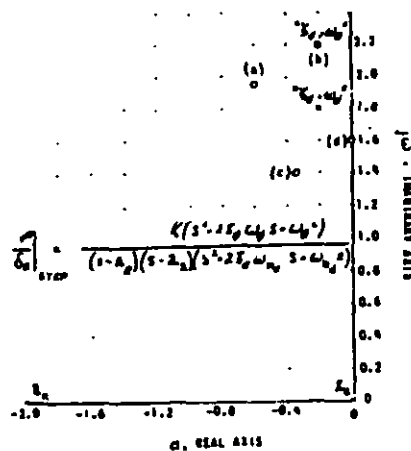
\phi|_{\text{STEP}} TRANSFER FUNCTION
