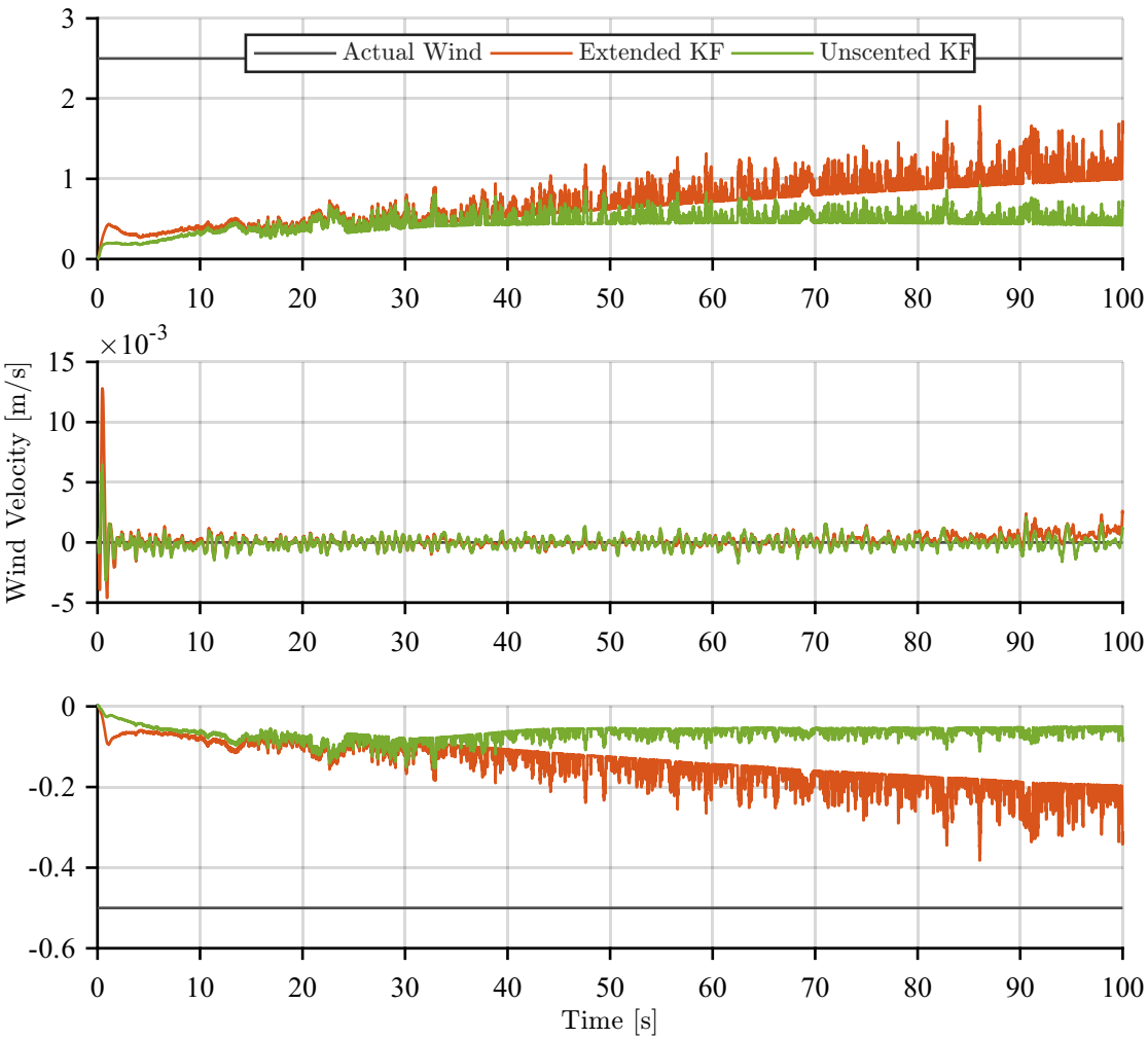
Actual and Estimated Wind in E_x/E_y/E_z -Direction
