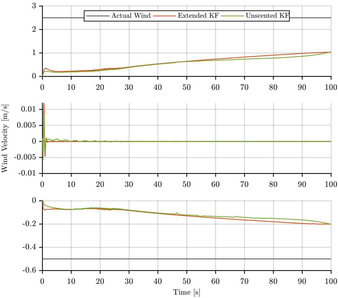
Actual and Estimated Wind in E_x/E_y/E_z -Direction
