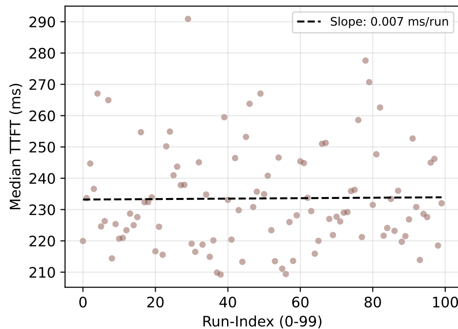
Mistral: Run-Index vs TTFT
