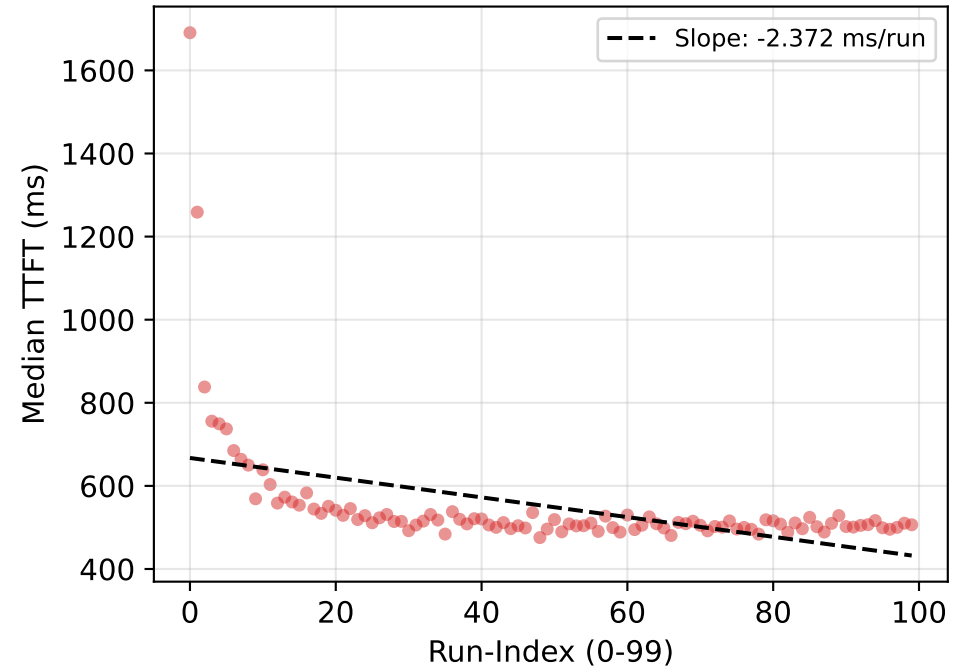
Openai: Run-Index vs TTFT
