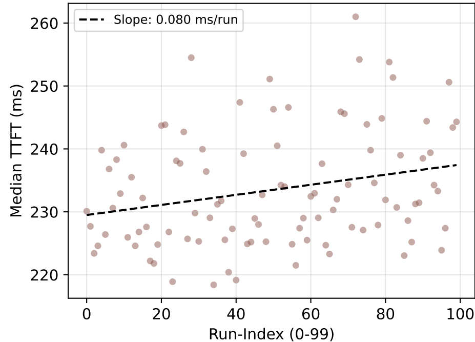
Mistral: Run-Index vs TTFT
