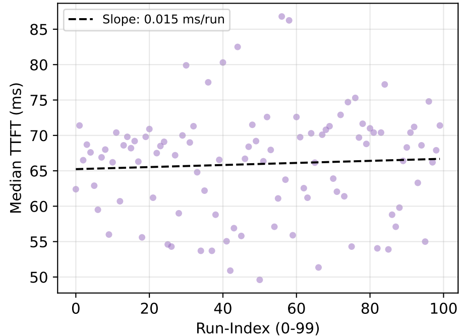
Groq: Run-Index vs TTFT
