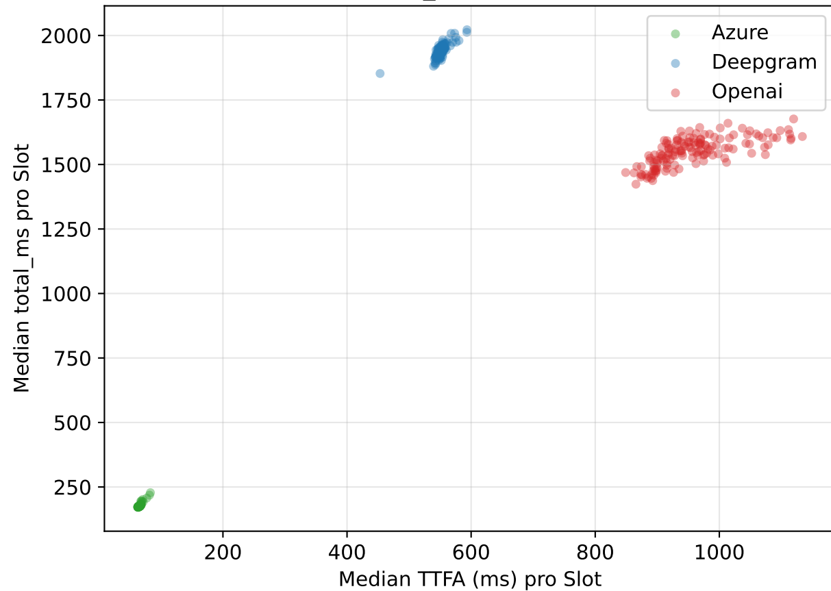
TTFA vs total_ms (je Slot-Median)
