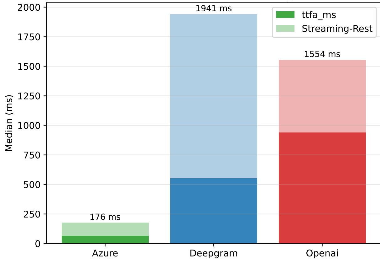
TTFA + Streaming-Rest = total_ms
