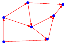
acyclic
