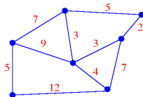
weighted
