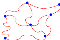
topological
