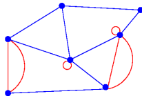
non-simple
