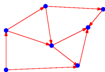
directed
