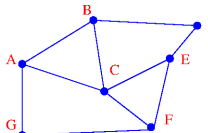
labeled
