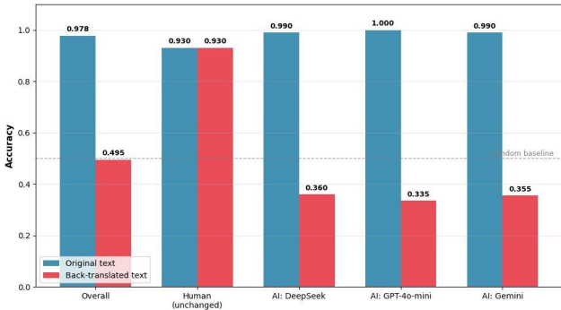
Detector Robustness Under Back-Translation Paraphrasing
