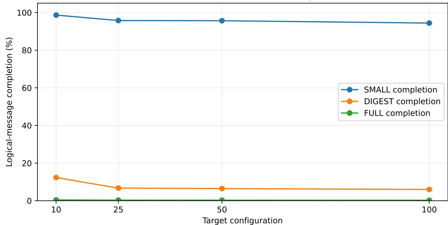
Final canonical-wire PHY/MAC completion
