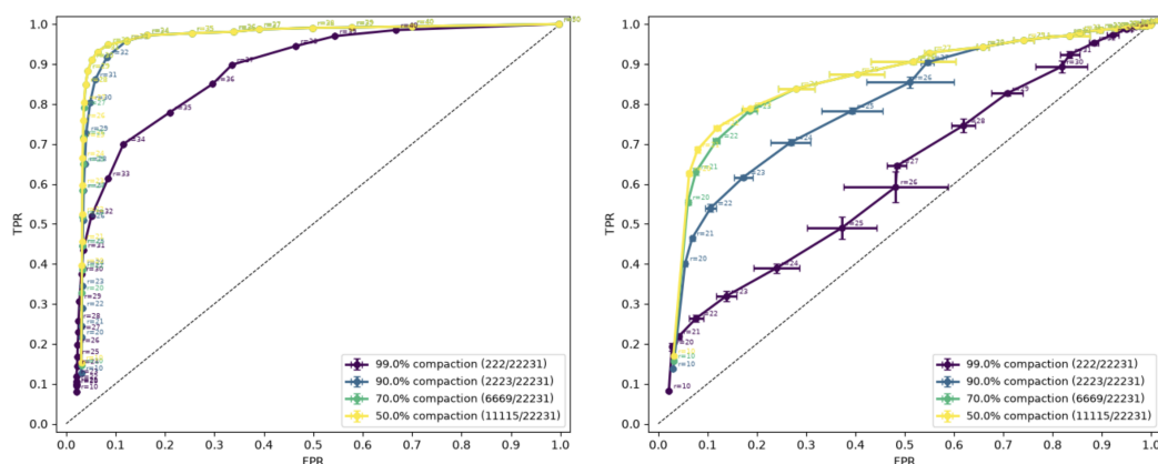
Figure 12: ROC Curves for UoS Radius Calibration. We show two representative curves, one for the gate projection (left) and one for the down projection (right), both in layer 17. Each curve color indicates different compaction rates (dictated by the maximal value of representative points M). The selected radius is the one with the maximal compaction rate, subject to being within the allowed TPR,FPR region (defined globally for all gates).
