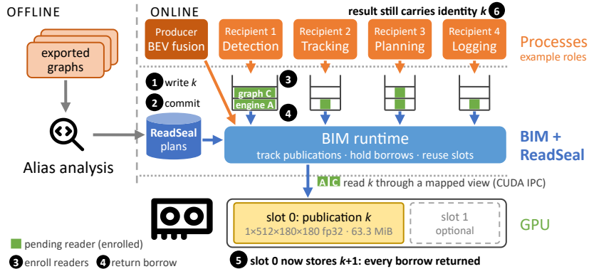
(a) BIM architecture and per-publication protocol
