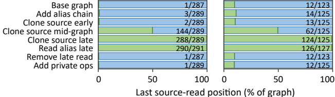
TransFusion head
