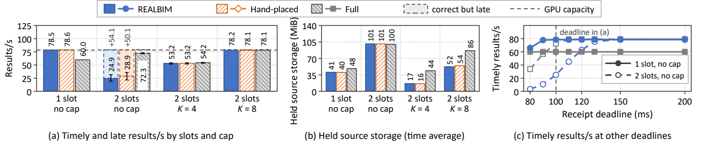
Fig. 7. One REALBIM slot matches full retention with two slots and an admission cap (30 Hz; six runs per condition and policy). K caps outstanding recipient requests; Hand-placed: standalone runtime. (a) Solid: timely results; dashed: correct but late; whiskers: 95% intervals. (b) Time-averaged source storage held by unreturned borrows. (c) The same runs re-scored at other deadlines.
