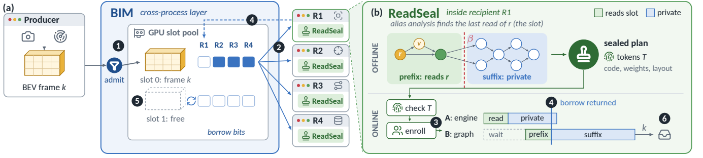
Fig. 3. REALBIM's two layers. (a) BIM, in the producer and shared memory, keeps a pool of GPU slots with one borrow bit per recipient and slot. (b) ReadSeal, inside each recipient: offline, alias analysis splits a reader's graph at its last read \beta of source r into a prefix that reads r and a private suffix, and tokens T bind the plan to code, weights, and input layout; online, the recipient checks T (also at each stage entry) and enrolls readers A, a TensorRT engine, and B, an exported graph. Numbers follow frame k (Section III).
