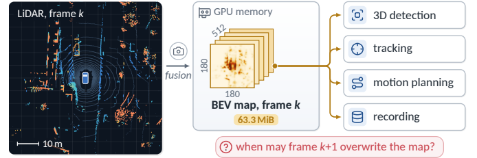
Fig. 1. One BEV map, four recipients. Fusing each LiDAR sweep (left, from nuScenes [5]) with camera images yields a 63.3 MiB map in GPU memory; its front face sketches one of 512 feature channels. Sharing the map avoids four copies, but the producer must decide when frame k+1 may overwrite it.
