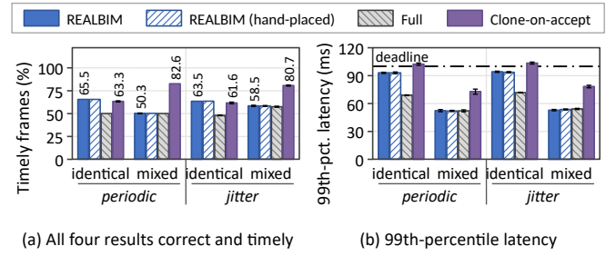
Fig. 8. Complete-frame delivery and tail latency with jitter and mixed recipients (30 Hz, one slot, no pipeline-wide cap; six runs per bar; whiskers: 95% t intervals; Hand-placed: REALBIM runtime ). (a) Share of the 900 scheduled frames per run whose four results are all correct and timely. (b) Per-run 99th-percentile latency of frames whose four results are all correct. Identical : four copies of the composition; mixed : four component profiles, one reading late with its last read at the graph's end .
