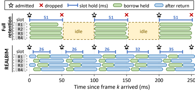
Fig. 4. Full retention refuses frames while the GPU idles. Measured one-slot trace at 20Hz; R1–R4 are the recipients, and labels give slot hold times in ms. Full retention's 51 ms hold just exceeds the 50ms period, so every other frame is refused. Under REALBIM, each recipient's work after its borrow return overlaps the next frame.
