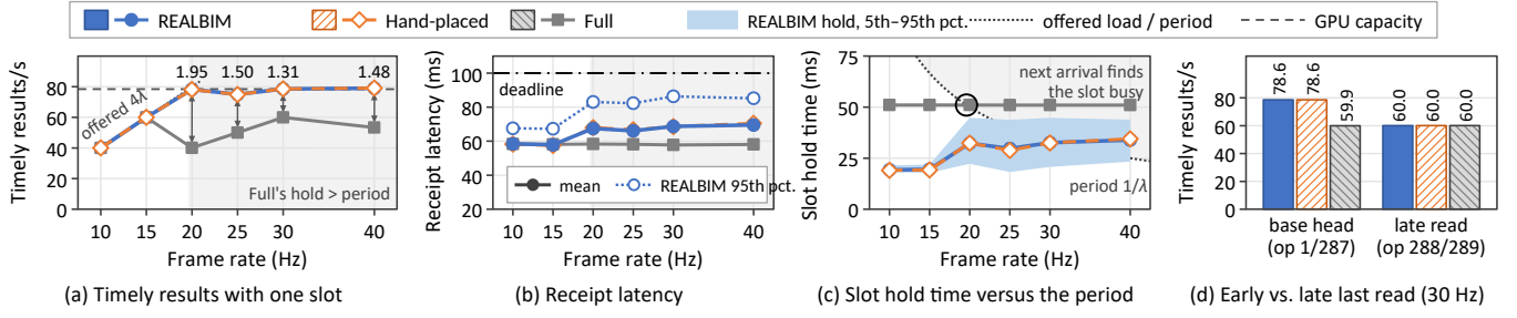
Fig. 6. Early reuse raises one-slot delivery under load, at a latency cost. One slot, no pipeline-wide cap K , six runs per condition and policy; each frame offers four recipient results. Hand-placed: standalone runtime releases at the same point as REALBIM by design (Section V). (a) Labels give REALBIM/Full ratios. (b) Mean receipt latency and REALBIM's mean per-run 95th percentile. (c) Mean hold and REALBIM's 5th–95th percentile; shading marks where Full's hold exceeds the frame period. (d) Moving the last read to the graph's end removes the gain.
