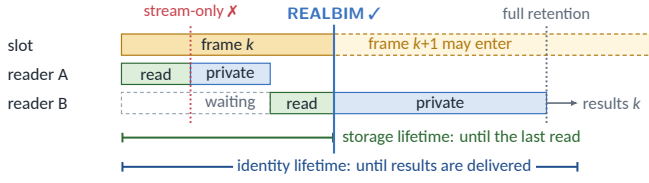
Fig. 2. Two lifetimes of one frame in a recipient with readers A and B. Storage is needed until B’s read, the last one; identity k , until results are delivered. Stream-only release frees the slot before B reads; REALBIM frees it at the last read, so frame k+1 can enter while B computes.
