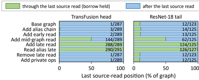
Fig. 5. Model edits move the last source read. Each bar is a graph snapshot that applies one edit to the base graph (Remove late read undoes Add late read). Green marks the operations up to the last source read, during which the recipient holds its borrow; labels give that operation's index/total operations.
