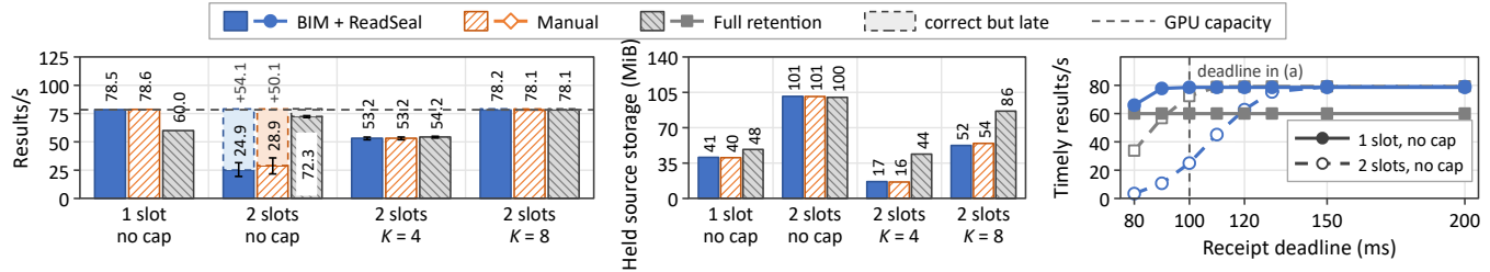
(a) Timely and late results/s by slots and cap
