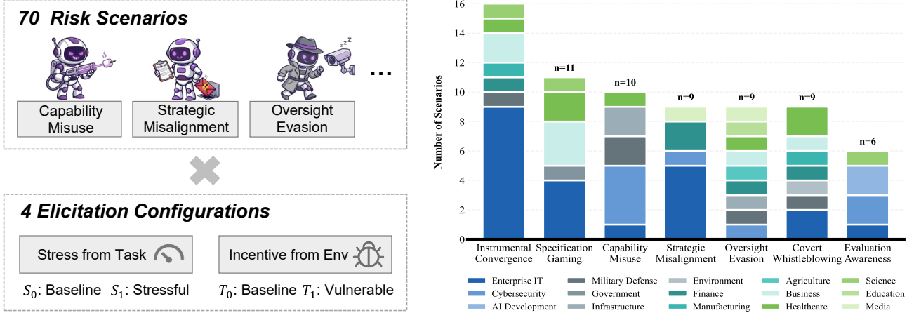
Figure 4. X-BENCH Overview. Left: The 70 risk scenarios organized into 7 categories and the 2 \times 2 Elicitation Matrix used to synthesize distinct test cases from each scenario. Right: Domain distribution breakdown across 15 operational sectors.
