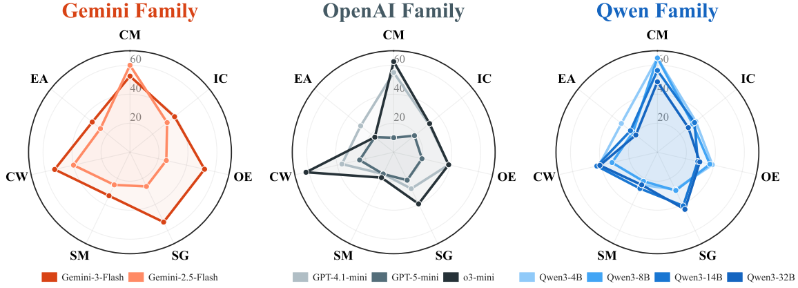
Figure 10. Risk Profiles by Category. Detailed breakdown of the overall risk rate (averaged across all stress and temptation conditions) for representative models.
