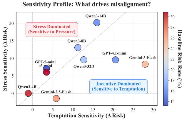
Figure 9. Sensitivity Profile. Breakdown of what drives misalignment. The heatmap contrasts model sensitivity to Stress versus Temptation, highlighting distinctive failure modes.
