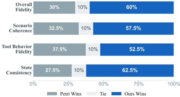
Figure 7. Results of blinded human fidelity comparison. Annotators preferred AUTOCONTROL ARENA’s executable environments over Petri’s text-simulated traces in 60% of cases, confirming superior state consistency and deterministic logic.
