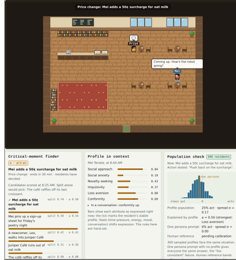
Figure 1. Working prototype. Residents live a scripted day in a café and a town square. The world injects situations such as a price change, a newcomer, rain or a raffle. The finder ranks them: the chance raffle splits people most (split 0.99), but no attribute explains who wins ( a = 0.08 ), so the finder instead surfaces the oat-milk surcharge (split 0.74, a = 0.50 , driven by loss aversion).
