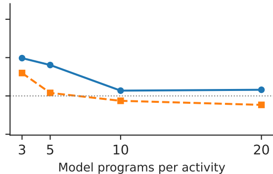
ESK Verbs
