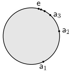
Figure 4.9: Discontinuity of fraction.
