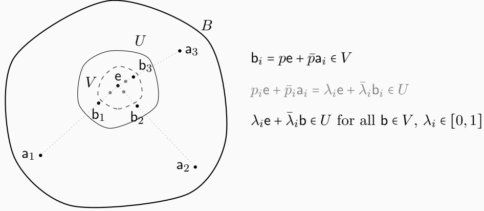
Figure 4.1: Boundedness shrinks all of A into the neighborhood V (giving the b_i ); the tube lemma guarantees that any further mixture of e with a point of V stays in U (giving the gray points).
