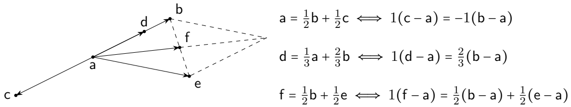
Figure 4.4: Once a reference point is picked (i.e. a in the figure), the differences with respect to that point behave like elements of a vector space. The relationship between ensembles in terms of mixtures become vector space relationships between differences. Note that the sum is effectively a “half parallelogram law,” so that the result always is a member of the convex space.
