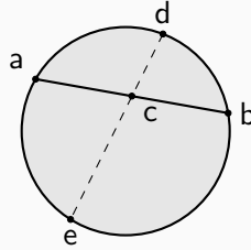
Figure 4.15: The set \{a, b\} is componential, but its convex hull (the segment) is not: c is in the convex hull but can be decomposed into d and e , which lie outside of the hull.
