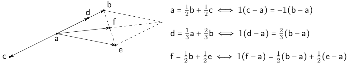
Figure 4.5: Once a reference point is picked (i.e. \mathbf{a} in the figure), the differences with respect to that point behave like elements of a vector space. The relationship between ensembles in terms of mixtures become vector space relationships between differences. Note that the sum is effectively a “half parallelogram law,” so that the result always is a member of the convex space.
