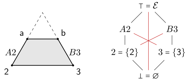
Figure 4.12: On the left, the cut triangle. On the right, the lattice of the orthogonal subspaces. The red lines connect the orthogonal complements.
