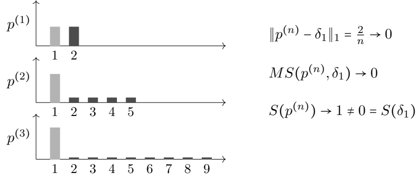
Figure 4.14: A vanishing fraction of probability mass spread over exponentially many outcomes. The distributions converge to \delta_1 in \ell^1 /total variation/Jensen–Shannon divergence, but the entropy does not converge.
