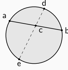
Figure 4.16: The set \{a, b\} is componential, but its convex hull (the segment) is not: c is in the convex hull but can be decomposed into d and e , which lie outside of the hull.
