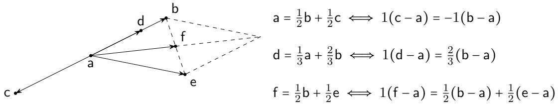
Figure 4.3: Once a reference point is picked (i.e. \mathbf{a} in the figure), the differences with respect to that point behave like elements of a vector space. The relationship between ensembles in terms of mixtures become vector space relationships between differences. Note that the sum is effectively a “half parallelogram law,” so that the result always is a member of the convex space.
