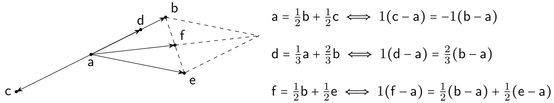
Figure 4.5: Once a reference point is picked (i.e. a in the figure), the differences with respect to that point behave like elements of a vector space. The relationship between ensembles in terms of mixtures become vector space relationships between differences. Note that the sum is effectively a “half parallelogram law,” so that the result always is a member of the convex space.
