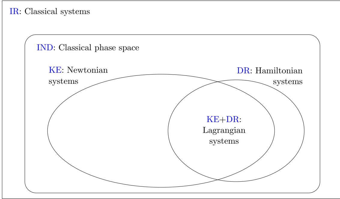
Figure 1.10: Relationship between the constitutive assumptions and the different formulations of classical mechanics. All classical systems satisfy infinitesimal reducibility. The independence of DOF recovers classical phase space. An ideal gas, with state variables [PVT] is an example of a classical system that does not satisfy IND. Another example is a system with non-holonomic constraints. Newtonian systems are fully characterized by spatial trajectories. Hamiltonian systems are characterized by deterministic and reversible dynamics. Lagrangian systems are characterized by both.
