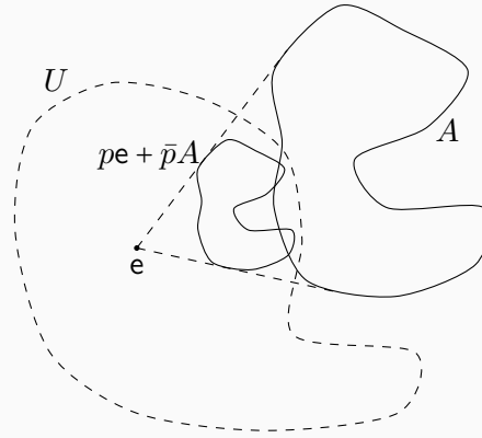
Figure 4.1: The set A is bounded around e as we can “shrink it” inside any open neighborhood U by using convex combinations.
