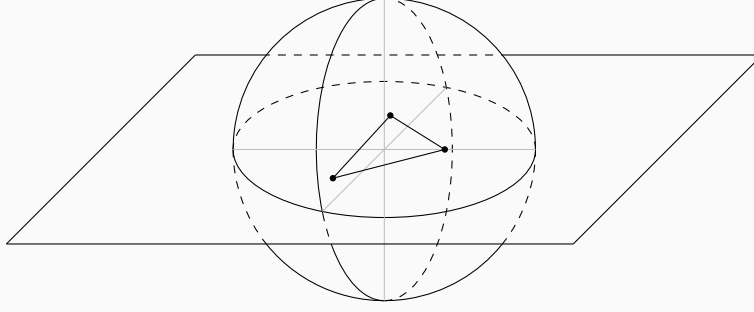
Figure 4.6: Affine vs. convex set. The ball is the ensemble space. The triangle represents a convex subset. The disc containing the triangle is the affine hull of the triangle in the ensemble space. The plane is the affine hull/span of the triangle in the embedding vector space centered at one of the three ensembles.
